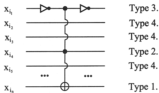
Figure 3.3: A single gate
