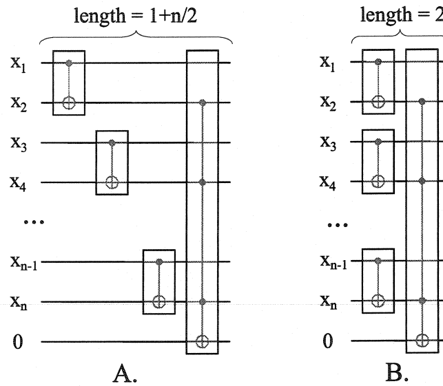
Figure 3.7: Reversible design structure.
