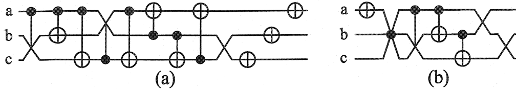
Figure 5.3: Circuits.
