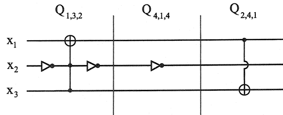
Figure 3.4: Circuit
