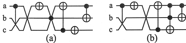
Figure 5.11: Simplified networks.
