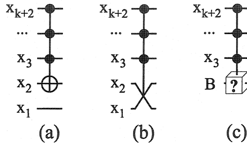
Figure 5.1: Toffoli, Fredkin and box gates.
