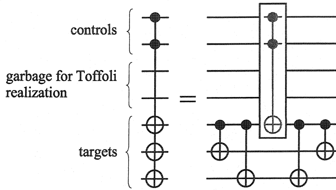
Figure 6.2: Construction of a single mEXOR gate.
