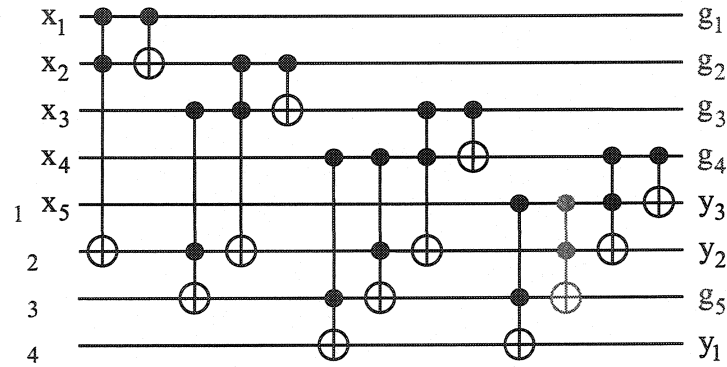
Figure 7.1: Circuit for rd53
