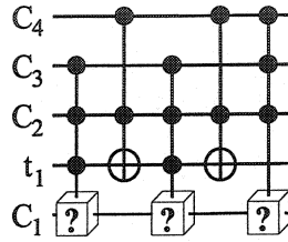
Figure 5.9: Class ATATB .
