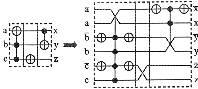
Figure 5.2: Transformation of a Toffoli circuit to a NOT-Fredkin circuit.
