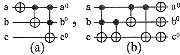
Figure 4.2: Circuits for the function shown in Table 4.2
