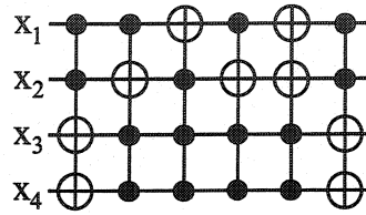
Figure 6.3: mEXOR gate network.
