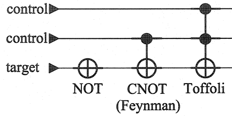
Figure 2.2: NOT, CNOT and Toffoli gates
