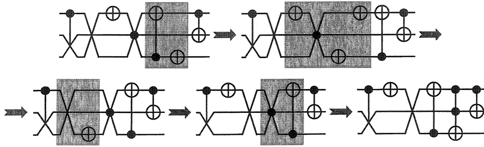
Figure 5.12: Simplifying one network into the other.
