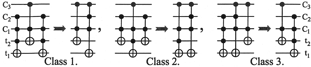
Figure 4.4: Toffoli templates.
