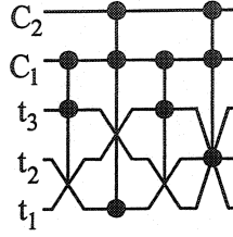
Figure 5.8: Link group.
