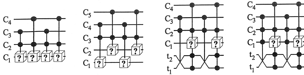
Figure 5.5: Class ABAB.
