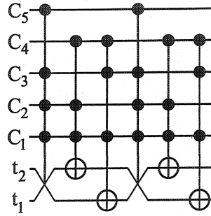
Figure 5.10: Class FTTFTT .
