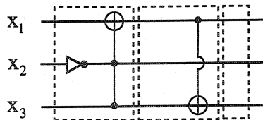
Figure 3.5: Pruned circuit
