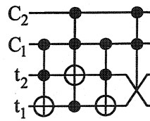
Figure 5.7: Fredkin definition group.
