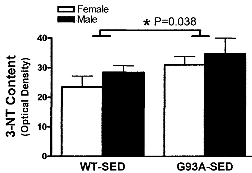
Figure 3.46 The level of nitrotyrosine (3-NT) in the DG of WT-SED and G93A-SED mice. G93A-SED mice had a higher 3-NT content than WT-SED mice, * p=0.038 , n=7-11 per group. Males had a trend to have high 3-NT content than females ( p=0.076 ). Data are means \pm SEM.
