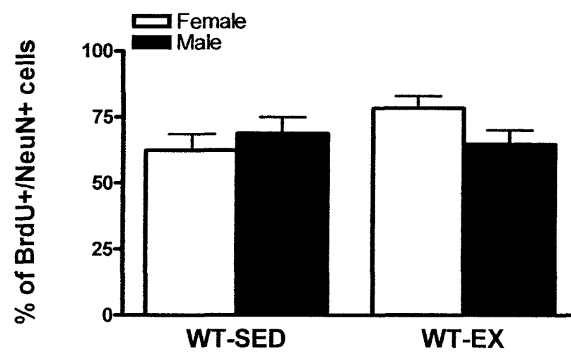
Figure 3.11 The neuronal differentiation of BrdU labeled surviving cells in the DG of WT-SED and WT-EX mice. There was no significant difference in the percentage of BrdU and NeuN double labelled cells between WT-EX and WT-SED mice, n=5-6 per group. Data are means \pm SEM.
