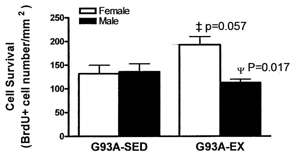
Figure 3.8 Cell survival in the dentate gyrus (DG) of G93A sedentary (G93A-SED) and G93A exercising mice (G93A-EX). Male EX mice had significantly (41.5%) fewer surviving cells than female EX mice G93A female EX mice had a trend to have 31.6% more surviving cells than G93A female SED mice. \Psi G93A-M-EX < G93A-F-EX, p=0.017 ; \ddagger a trend, G93A-EX females > G93A-SED females, n=10 per group except for G93A-SED females =11. Data are means \pm SEM.
