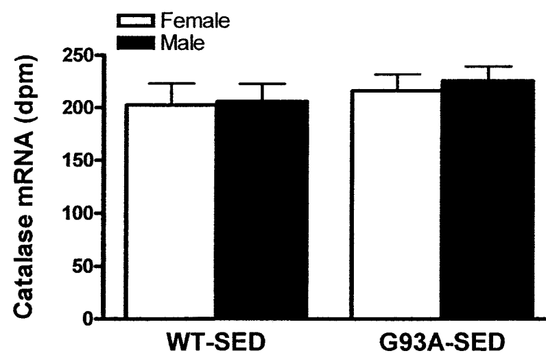
Figure 3.34 The expression of catalase mRNA in the DG of WT-SED and G93A-SED mice. There is no significant difference between WT-SED and G93A-SED mice, n=11-13 per group. Data are means \pm SEM.
