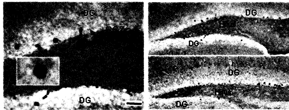
Figure 3.5 Representative images of BrdU labeled surviving cells in the dentate gyrus (DG) of wild type (WT) and G93A mice. (A) A representative image showed that most surviving cells were located in the DG, with more rounded nuclei, sometimes with the typical chromatin structure of granular cells (insert). Representative images showed surviving cells in G93A mice (B) than in WT mice (C). Scale bar = 25 \mu m in A, 100 \mu m in B,C. G93A mice, n=21; WT mice, n=23.
