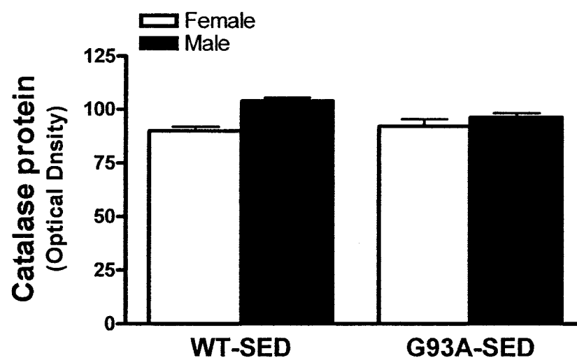
Figure 3.38 The content of catalase in the DG of WT-SED and G93A-SED mice.
