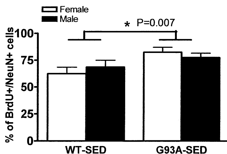
Figure 3.10 The neuronal differentiation of BrdU labeled surviving cells in the DG of WT and G93A mice. The percentage of double labelled BrdU and NeuN cells was 22.4% higher in G93A-SED than in WT-SED collapsed across sex. *G93A-SED>WT-SED, p = 0.007 , n=5-6 per group. Data are means \pm SEM.
