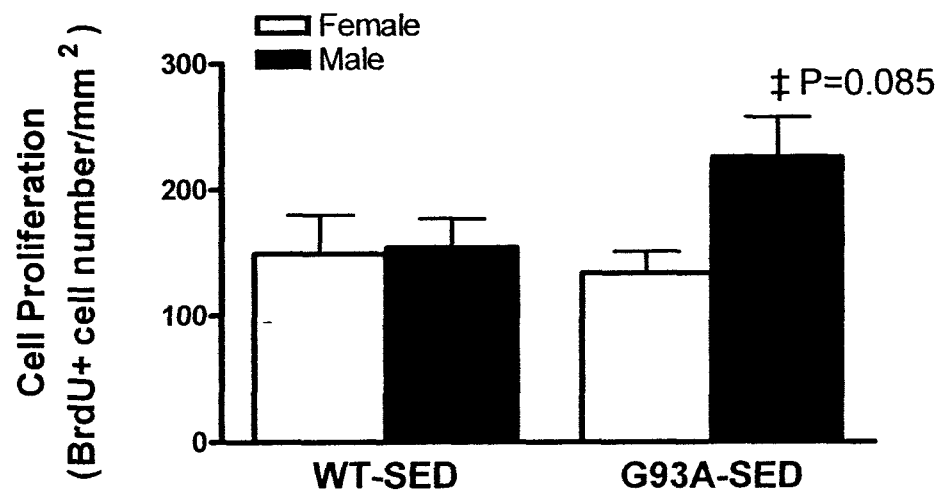
Figure 3.2 Cell proliferation in the dentate gyrus (DG) of wild type (WT-SED) and G93A (G93A-SED) sedentary mice. G93A mice had 18.5% more proliferating cells than WT mice collapsed across sex, due to 68.7% greater number of proliferating cells in G93A males vs G93A females (§ a trend, G93A-M-SED > G93A-F-SED , p=0.085 , n = 6 per group). Data are means \pm SEM.
