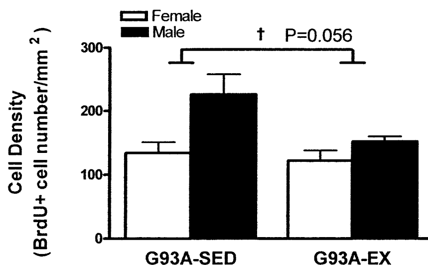
Figure 3.4 Cell proliferation in the dentate gyrus (DG) of G93A sedentary (G93A-SED) and G93A exercise mice (G93A-EX). EX mice had 24.4% fewer proliferating cells vs SED mice, due to 32.7 % fewer proliferating cells in EX males vs. SED males. † G93A-EX < G93A-SED, p=0.056 , n = 6 per group except for G93A EX males = 5. Data are means \pm SEM.
