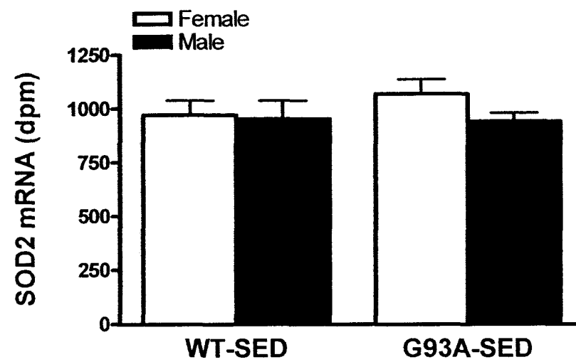
Figure 3.26 The expression of SOD2 mRNA in the DG of WT-SED and G93A-SED mice. There was no significant difference in DG SOD2 mRNA expression between WT-SED and G93A-SED mice, n=11-13 per group. Data are means \pm SEM.
