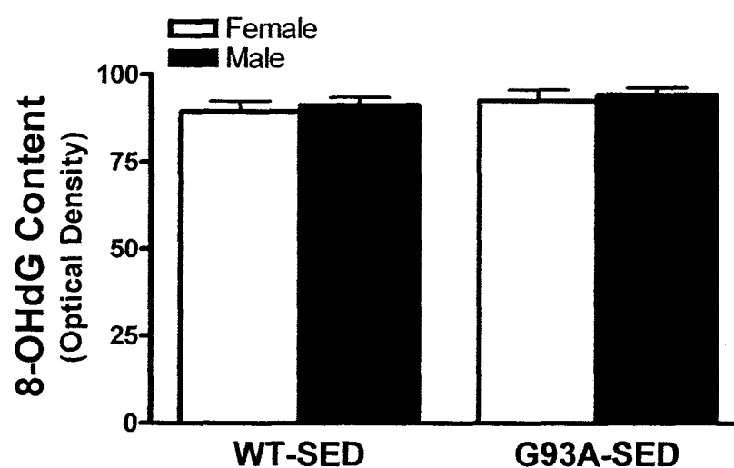
Figure 3.42 The content of 8-OHdG in the DG of WT-SED and G93A-SED mice.
