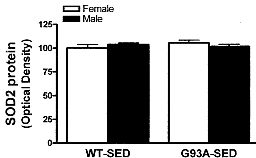
Figure 3.30 The content of SOD2 protein in the DG of WT-SED and G93A-SED mice. There was no significant difference in DG SOD2 protein content between WT-SED and G93A-SED mice, n=9-11 per group. Data are means \pm SEM.
