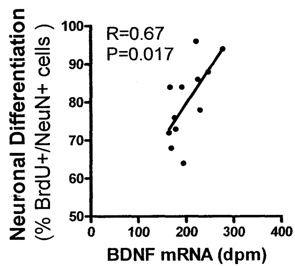
Figure 3.24 Correlation between DG BDNF mRNA and neuronal differentiation of BrdU labeled surviving cells in G93A-EX mice. In G93A-EX mice, DG BDNF mRNA expression was significantly and positively related to neuronal differentiation of BrdU labeled surviving cells ( r=0.67 , p=0.017 , n=11 ). Data are means \pm SEM.
