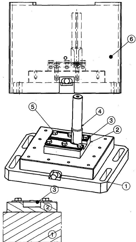
Fig. 1 Experimental setup design for measuring machining dust during orthogonal milling process—1: Three axes dynamometer; 2: Support; 3: 6061-T6 aluminum workpiece; 4: Cutting tool; 5: Fixture screw; and 6: dust cover
