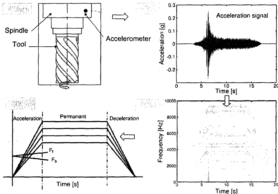
Fig. 1. Different steps for spectrogram analysis (Step 1) Experimental setup: end mill with an accelerometer on the free-end of the spindle, followed by a spindle rotation for a short time period (Step 2) Collected acceleration signal (Step 3) Spectrogram analysis of the acceleration–deceleration period time (Step 4) Interpretation of the spectrogram results: F_f forward frequency and F_b backward frequency (see [23] for more details).
