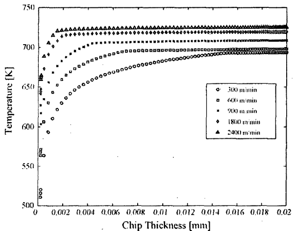
Fig. 12 – Simulated temperature in the secondary shear zone versus chip thickness for 7075-T6 aluminium for a half immersion up-milling test at different cutting speeds: 4 flutes, DOC=1.27 mm, f = 0.203 mm/min.
