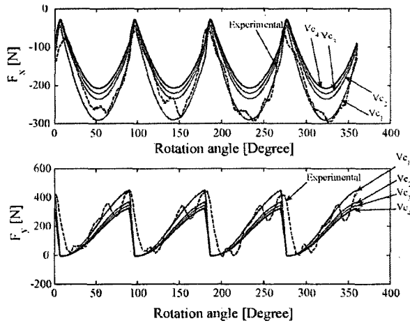
Fig. 9 – Influence of the cutting speed on the cutting forces for half immersion up-milling test 7075-T6: axial depth of cut (DOC)=2.54 mm, f = 0.203 mm/tooth, V_{c1} = 600 m/min, V_{c2} = 1200 m/min, V_{c3} = 1800 m/min, V_{c4} = 2400 m/min, experimental test (dashed line) at 600 m/min.
