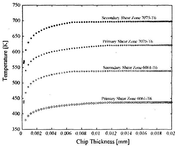
Fig. 10 – Simulated temperature in the primary and the secondary shear zone versus the chip thickness for 7075-T6 and 6061-T6 aluminium for a half immersion up-milling test: 4 flutes, DOC=1.27 mm, f = 0.203 mm/min, V_c = 600 m/min.
