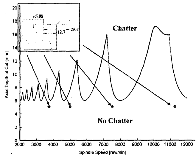
Fig. 6. Choosing of stable cutting conditions using the stability lobes. The dots represent the cutting conditions reported in Table 2 (dimensions are in mm). The considered material is the 7075-T6 aluminum alloy.
