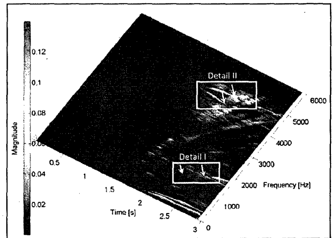
Fig. 2. Visualization of the influence of the spindle speed on the machine tool natural frequencies from spectrogram analysis. Arrows indicate an intersection between the machine tool natural frequency and the spindle revolution frequency.
