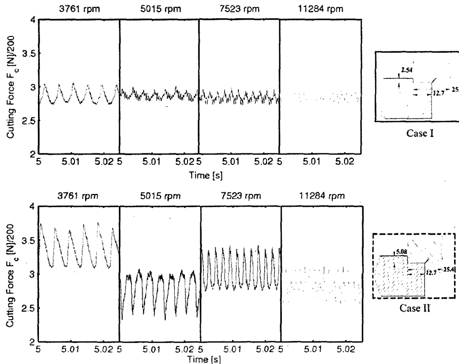
Fig. 14. Experimental verification of absolute stability for two cases using the amplitude of the cutting force F_c . Observe the very slight change in the cutting force for Case I for different spindle speeds at a constant depth of cut (2.54 mm).
