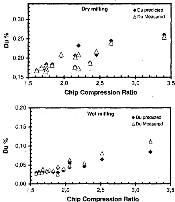
Fig. 12 Effect of chip compression ratio on predicted and measured dust generation
