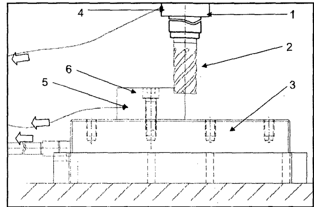
Fig. 5. Schematization of the experimental setup: 1—non-rotative part of the spindle, 2—a three flute carbide end mill, 3—Kistler dynamometer [9255-B], 4—accelerometer #1 (PCB 352C34), 5—accelerometer #2 (PCB 352C34), 6—work-piece AA7075-T6. Arrows indicate the data transfer to the Matlab-based data acquisition system.
