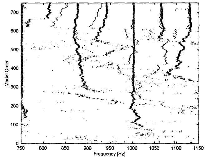
Fig. 10. Frequency stability diagram using the least square complex exponential method (LSCE) method, the treated signals are from test #1. The black cross-symbols (+) present the results in the x direction; the red dot symbols (.) present the results in the y direction.
