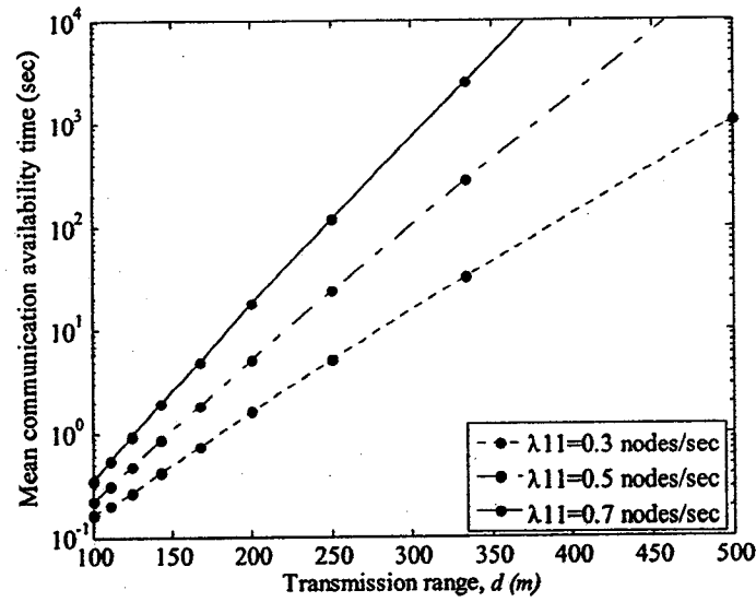
Fig. 5.14. Mean communication availability time for the path \Omega_1 , as a function of transmission range, with arrival rate \lambda_{11} as a parameter and maximum mean speed v_0 = 25 m/s.
