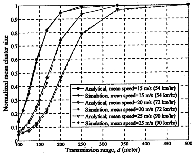
Fig. 4.4. Normalized mean cluster size seen by a new arrival as a function of transmission range with mean node speed as a parameter.
