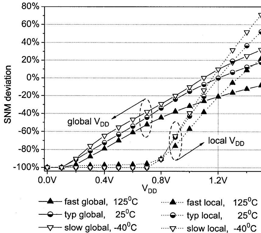
Figure 3.19 SRAM cell SNM deviation vs. V_{DD}
