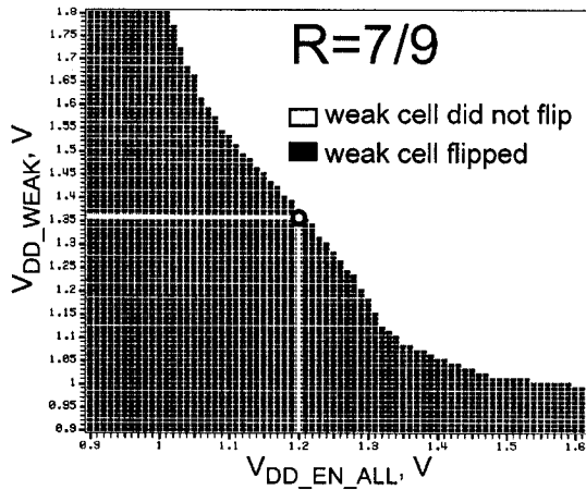
(c) Shmoo plot for R = 7/9 ; a circled dot represents the detection threshold for V_{DD\_EN\_ALL} = 1.2V .
