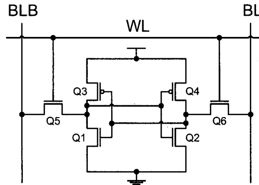
Figure 2.3 Six-transistor (6T) CMOS SRAM cell.
