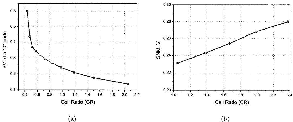
Figure 2.5 The rise \Delta V of the "0" node (a) and the SNM (b) as a function of the Cell Ratio (CR) ( CR = \frac{W_1}{L_1} / \frac{W_5}{L_5} = \frac{W_2}{L_2} / \frac{W_6}{L_6} in Figure 2.3) in a 6T CMOS SRAM cell (simulated in CMOS 0.13\mu m technology, V_{DD}=1.2V ).
