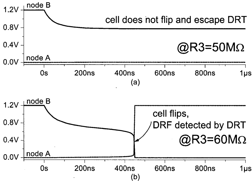
Figure 4.6 Data Retention Fault due to the discharge of node B through the off-state current of Q2 (simulation results for CMOS 0.13 \mu\text{m} technology, V_{DD}=1.2\text{V} , T=150^\circ\text{C} ). A resistive open R3=50\text{M}\Omega is insufficient to flip the cell and thus is not detected by Data Retention Test (DRT) (a), whereas R3=60\text{M}\Omega causes a DRF and is detected by DRT (b).
