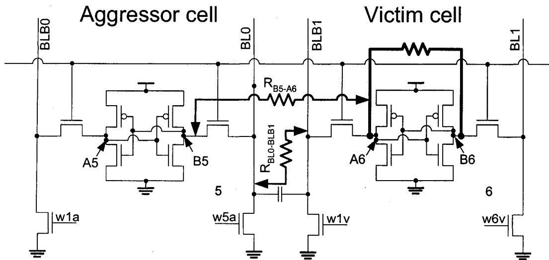
Figure 5.7 An excerpt of Figure 5.1 on page 110 showing the coupling resistive bridge defects ( R_{B5-A6} and R_{BLO-BLB1} ) and inter-bit-line capacitance between the bit lines of the aggressor and the victim cells.
