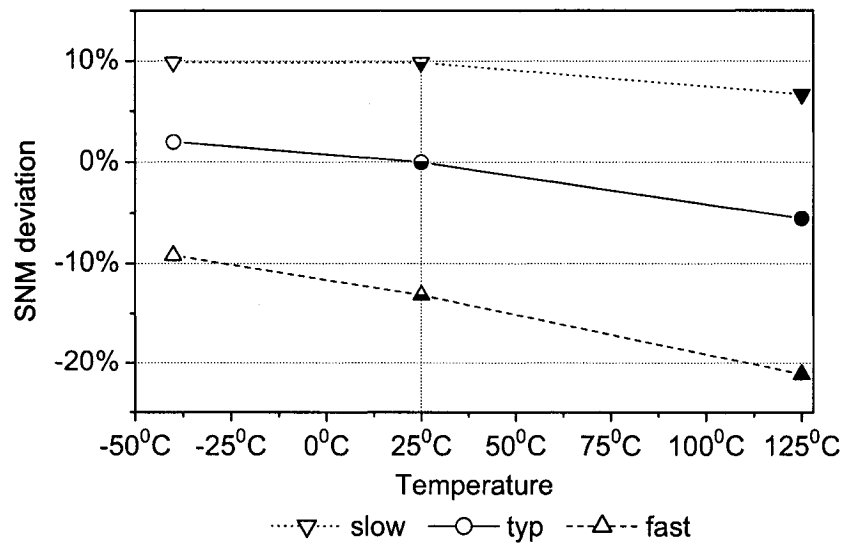
Figure 3.21 SRAM cell SNM deviation vs. temperature
