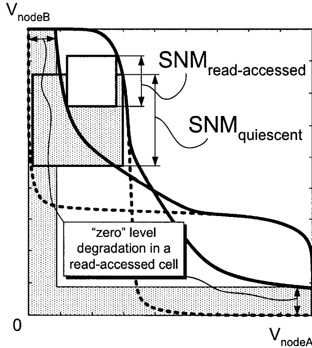
Figure 3.11 Simulated VTCs of a 6T SRAM cell in retention (quiescent) and in the read-accessed modes (CMOS 0.18\mu m ). Note that the read-accessed SNM is about a half of that in the retention mode.
