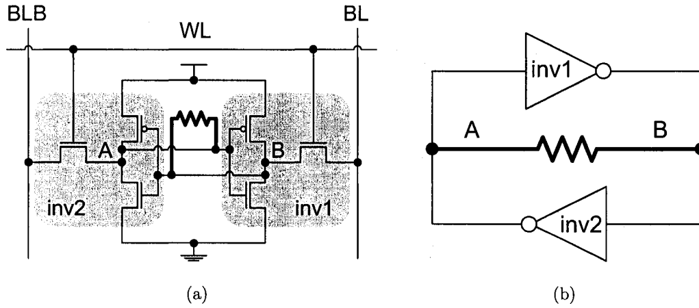
Figure 4.9 Proposed Weak Cell Fault Model (a) and its equivalent circuit (b).
