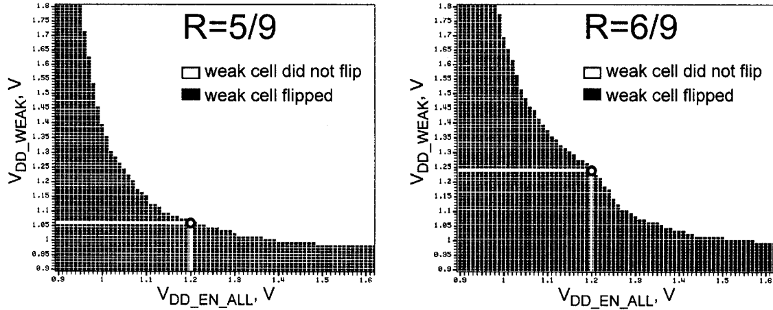
(a) Shmoo plot for R = 5/9 ; a circled dot represents the detection threshold for V_{DD\_EN\_ALL} = 1.2V . (b) Shmoo plot for R = 6/9 ; a circled dot represents the detection threshold for V_{DD\_EN\_ALL} = 1.2V .
