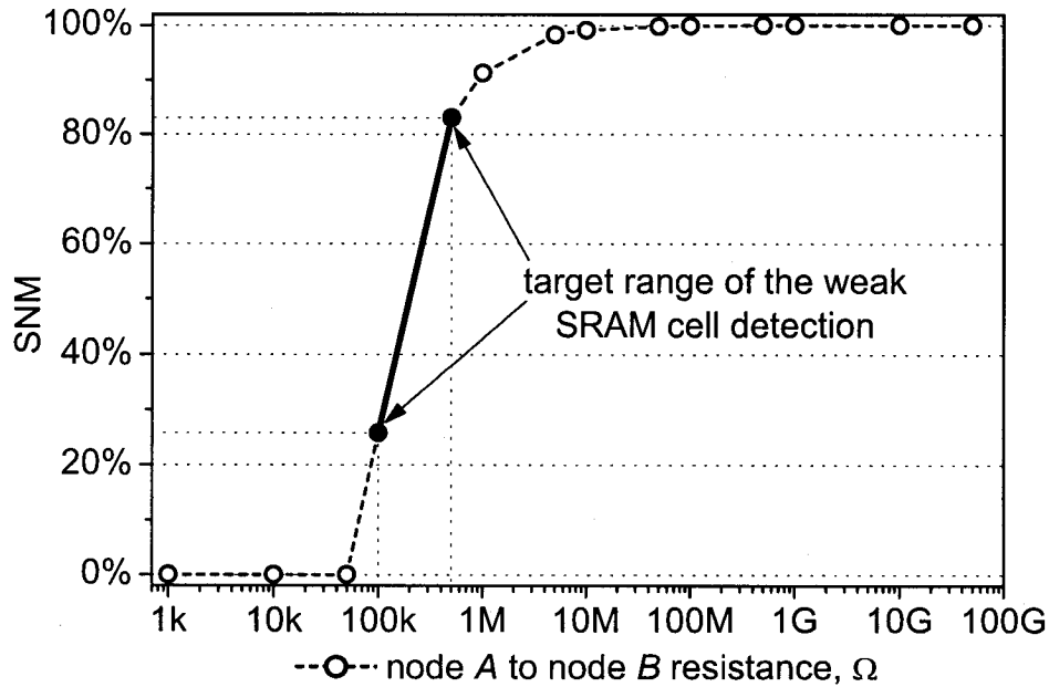
Figure 4.8 A possible target range of the SNM modelled by a given range of a resistor between node A and node B.
