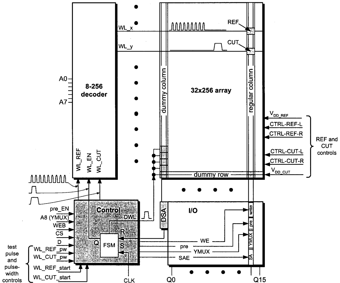
Figure 6.18 Block-level diagram of the WLPT test chip.
