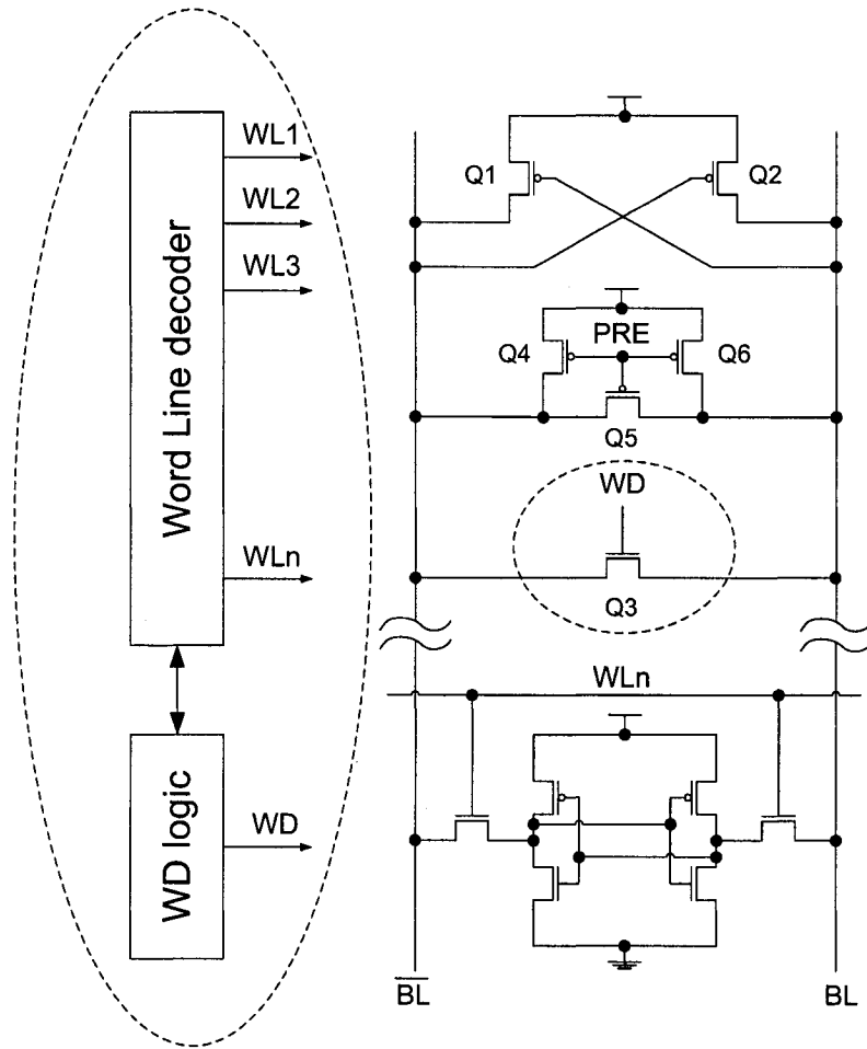
Figure 6.3 RCRPT hardware implementation
