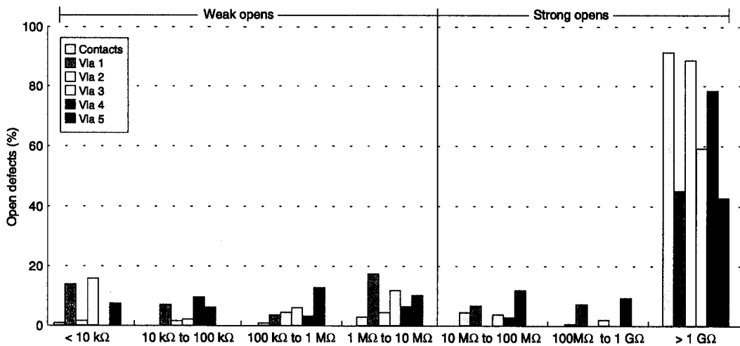
Figure 4.2 Resistance distribution for contact and via opens [6].
