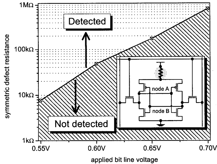
Figure 6.23 WLPT detection of a symmetric defect resistance in the pull-up path of an SRAM cell as a function of applied bit line voltage (CMOS 0.13 \mu m, C_{BL} = 400 fF).
