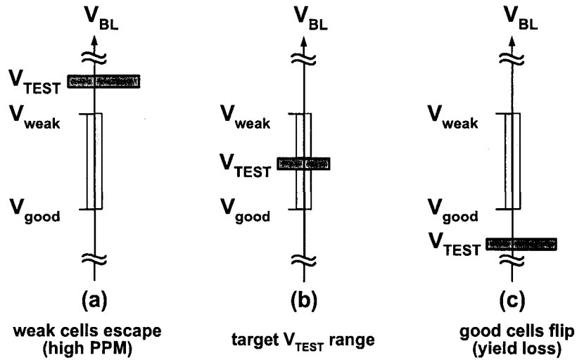
Figure 4.12 Programming V_{TEST} to set a correct pass/fail test threshold: (a) V_{TEST} is set too high, which causes the weak cells to escape (high PPM), (b) V_{TEST} is set correctly, (c) V_{TEST} is set too low, which causes the good cells to flip (yield loss).
