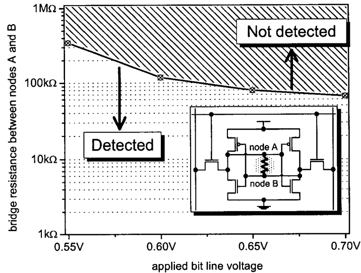
Figure 6.25 Detection of a resistive bridge between node A and node B (as per the proposed stability fault model introduced in Section 4.1.2) as a function of applied bit line voltage (CMOS 0.13 \mu\text{m} , C_{BL} = 400\text{fF} ).
