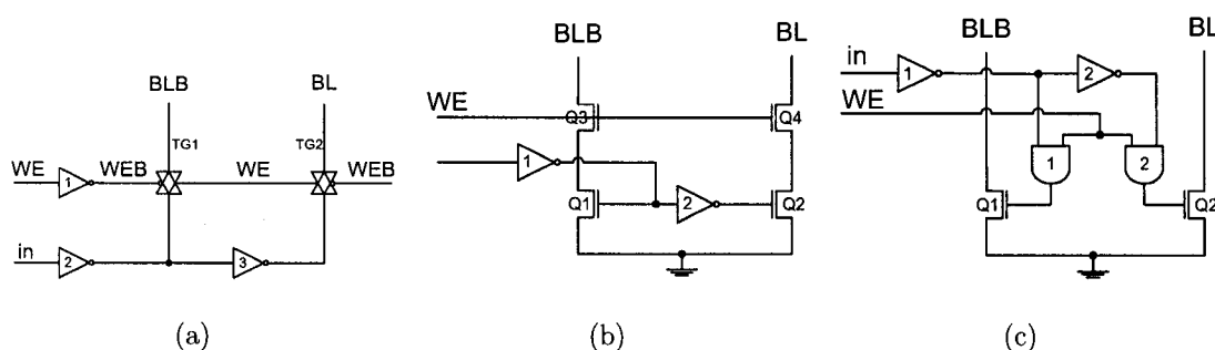
Figure 2.11 Write driver circuits.
