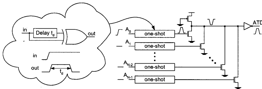
Figure 2.16 Address Transition Detector (ATD) [3].
