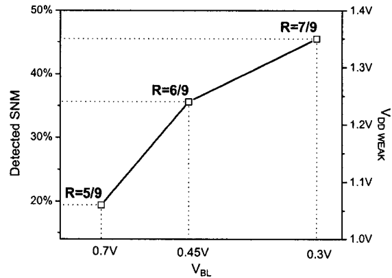
(d) Detection capability of the proposed DFT technique for V_{DD\_EN\_ALL} = 1.2V . Programming R from 5/9 to 7/9 changes the weak cells detection threshold from 18% to 46% of the nominal SNM.
