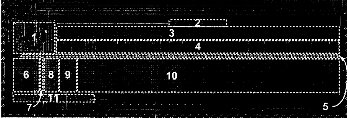
Figure 6.17 8Kb synchronous SRAM test chip with WLPT (IBM CMOS 0.13 \mu\text{m} 8 metal process): (1) control block, (2) decoder, (3) post-decoder, (4) word line drivers, (5) dummy column and dummy SA, (6) SAs, column MUXs, write drivers and precharge/equalization, (7) dummy row, (8) reference SRAM cells for WLPT, (9) weak SRAM CUTs for WLPT, (10) regular SRAM cells and (11) pad drivers.
