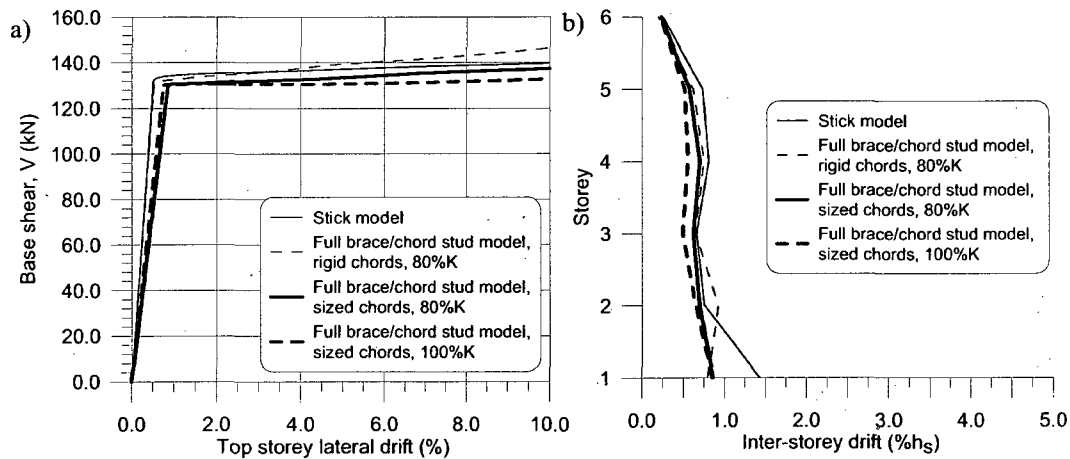
Figure 3.16: a) Pushover analysis and b) Mean Inter-storey drift comparison based on seven earthquake records for models 6S R d R 0 2.6-minbrace and 6S full brace/chord stud
