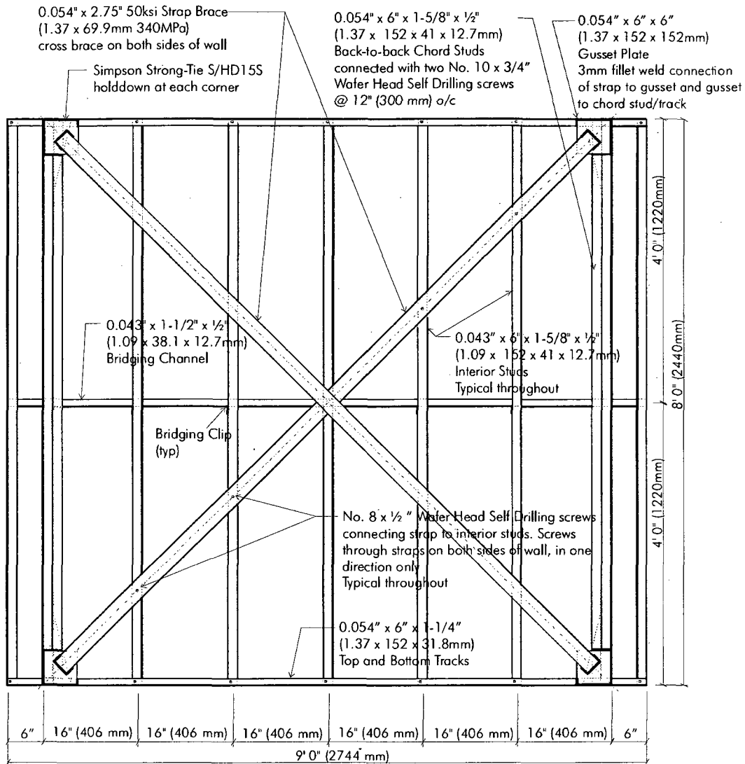
Figure B.34: Nominal dimensions and specifications for walls 17A-M and 18A-C
