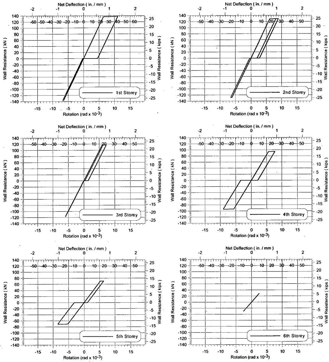
Figure H.2: Hystereses for each storey, CM earthquake record, model 6S R d R 0 2.6-minbrace
