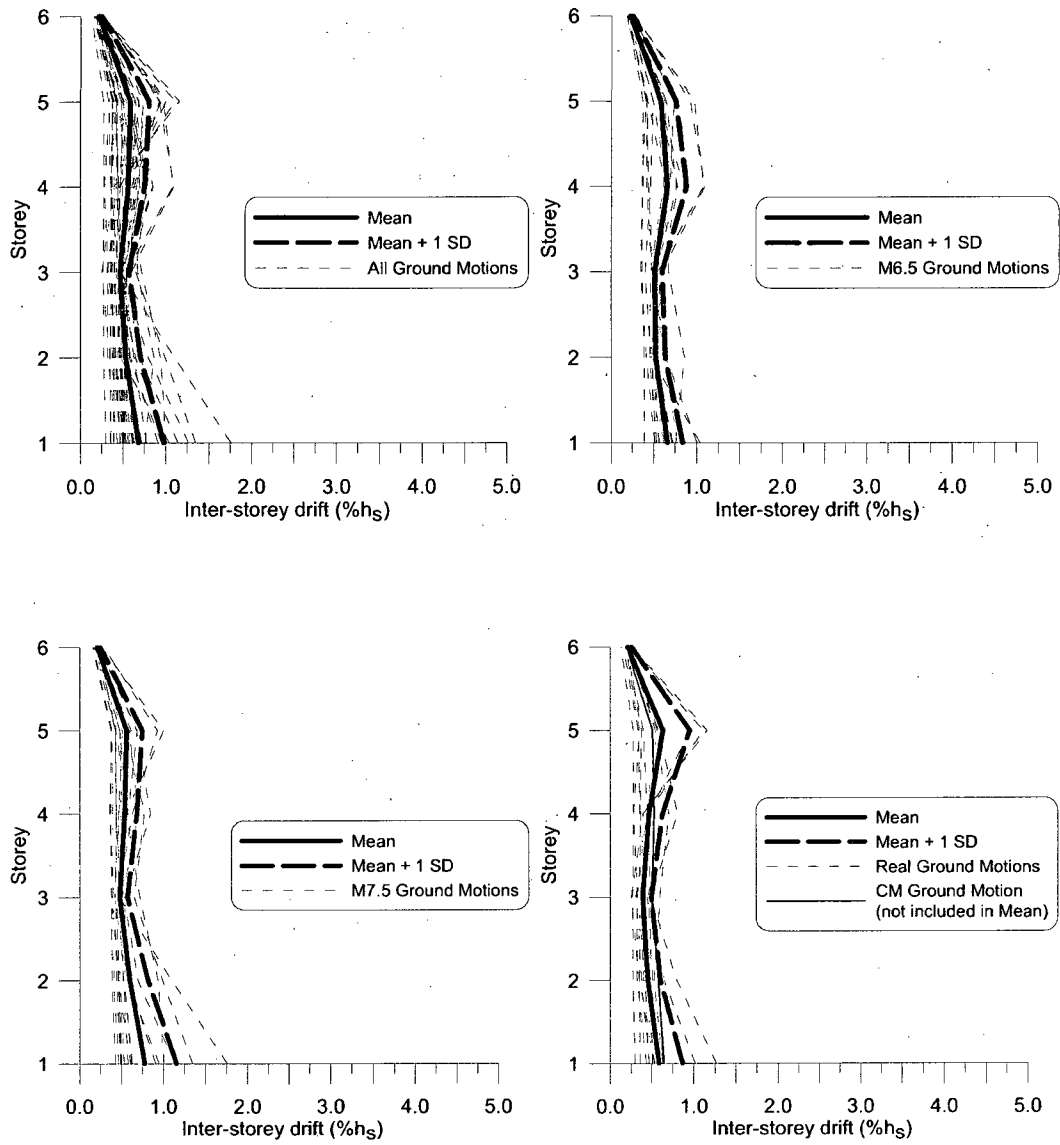
Figure I.2: Storey height versus inter-storey drift for 6S R o R o 2.6-minbrace sized 100% full brace/chord stud model
