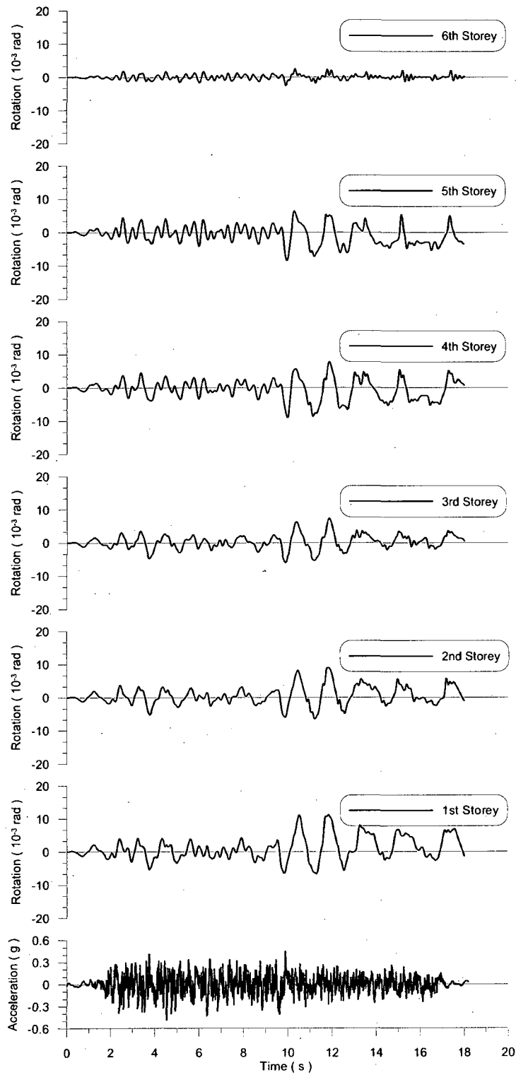
Figure H.4: Time history showing rotation vs. time for each storey, CM earthquake record, model 6S R 0 R 0 .2.6-minbrace
