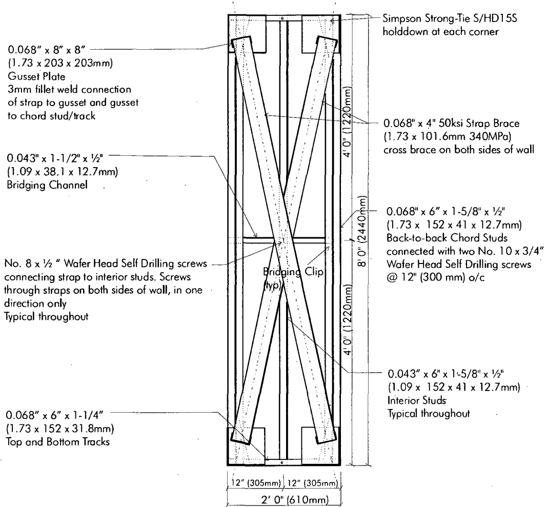
Figure B.40: Nominal dimensions and specifications for walls 23C-M and 24C-C
