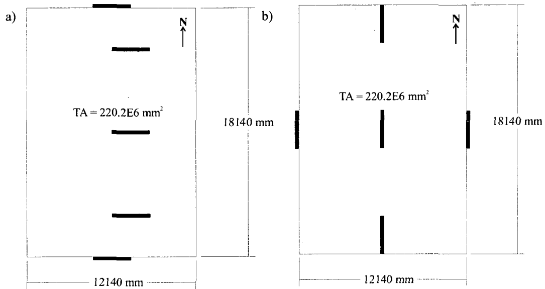
Figure 3.2: Braced wall location for model 6S R_dR_o2.6 -minbrace a) E-W direction earthquake, and b) N-S direction earthquake
