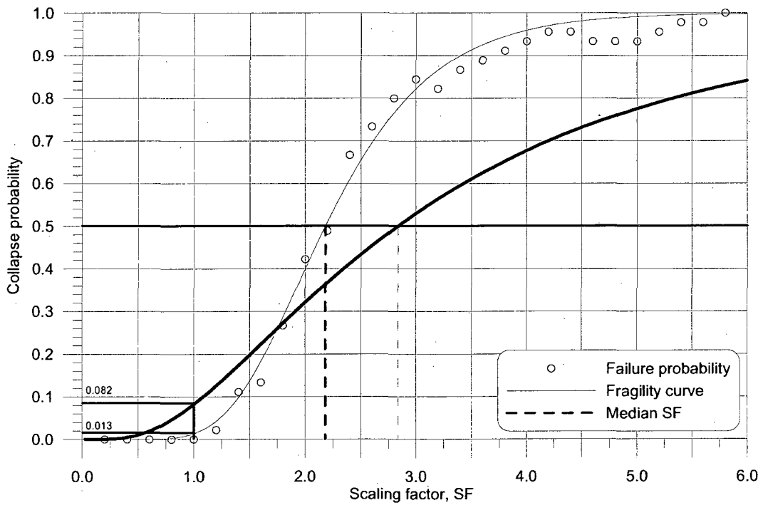
Figure I.18: Fragility curve for model 7S R_d R_o 2.6-2brace
