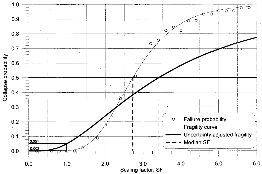
Figure I.10: Fragility curve for model 6S R_d R_o 2.6 -minbrace
