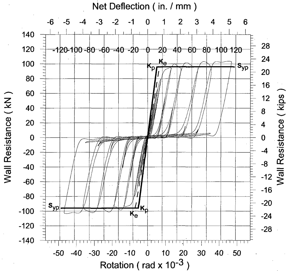
Figure A.25: Cyclic results for test 24A-C
