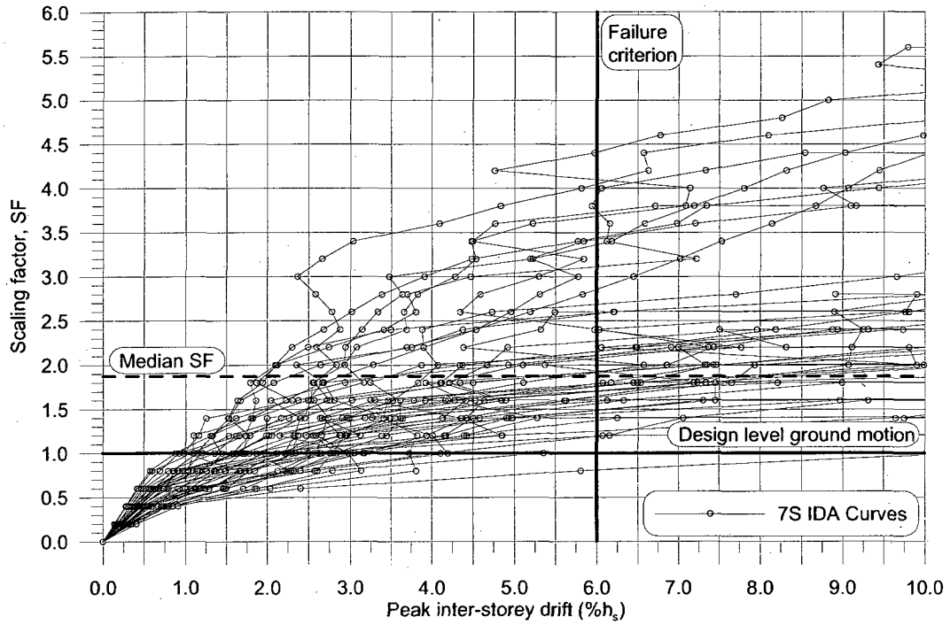
Figure I.19: IDA analysis for model 7S R 4 R 4 -minbrace
