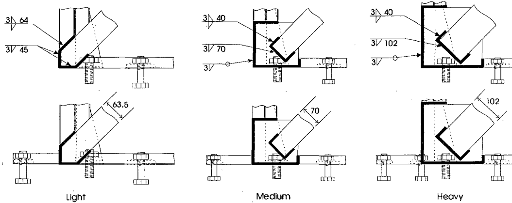
Figure 2.11: Corner details for 2440 x 2440mm light, medium and heavy walls
