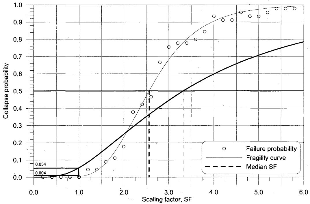
Figure I.16: Fragility curve for model 7S R_d R_o 2.6 -minbrace
