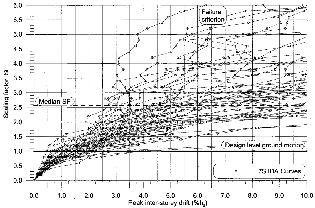
Figure I.15: IDA analysis for model 7S R_d R_o 2.6 -minbrace
