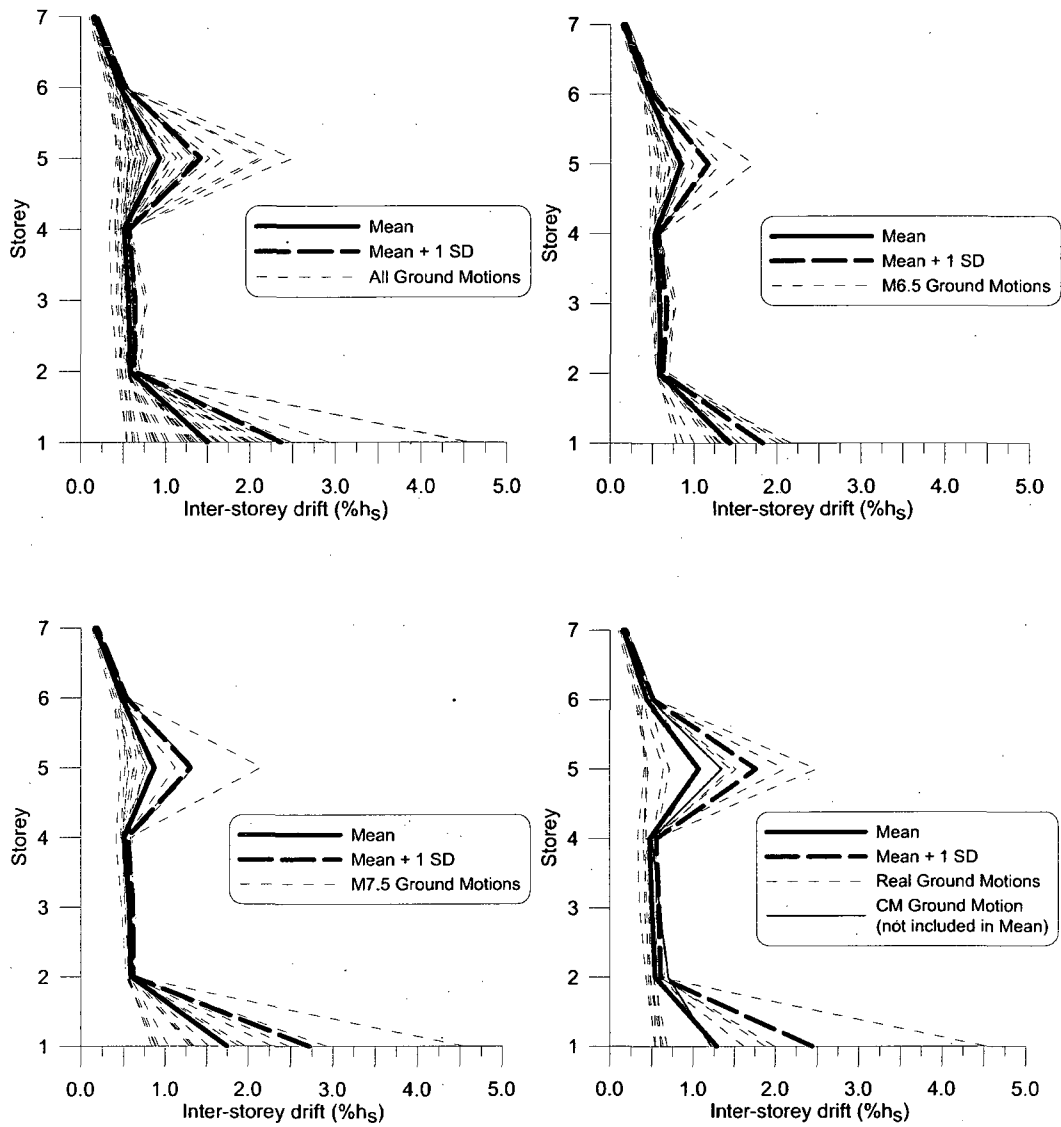
Figure I.7: Storey height versus inter-storey drift for 7S R 4 R 0.2.6 -2brace model
