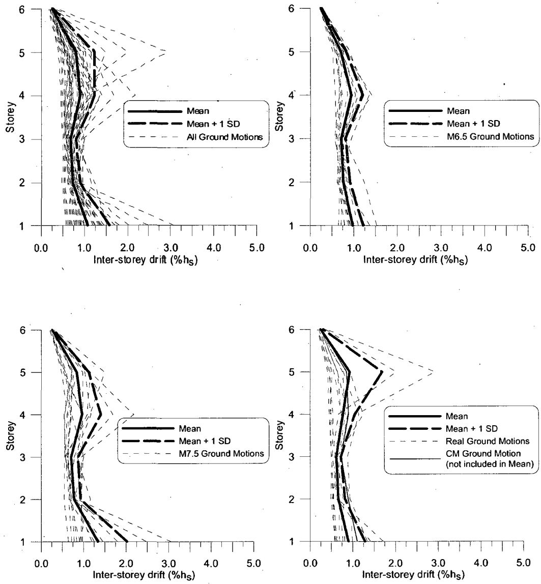
Figure I.3: Storey height versus inter-storey drift for 6S R 4 R 0.2.6 -minbrace model
