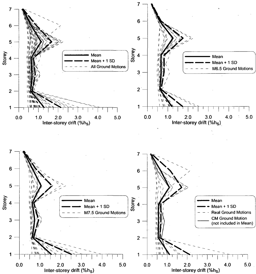
Figure I.6: Storey height versus inter-storey drift for 7S R 4 R 0.2.6 -minbrace model
