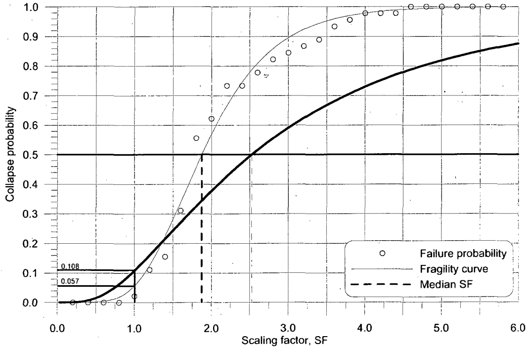
Figure I.20: Fragility curve for model 7S R 4 R 4 -minbrace
