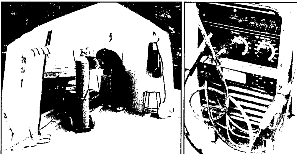
Figure 2.5: Welding setup and Lincoln Electric GMAW welder
