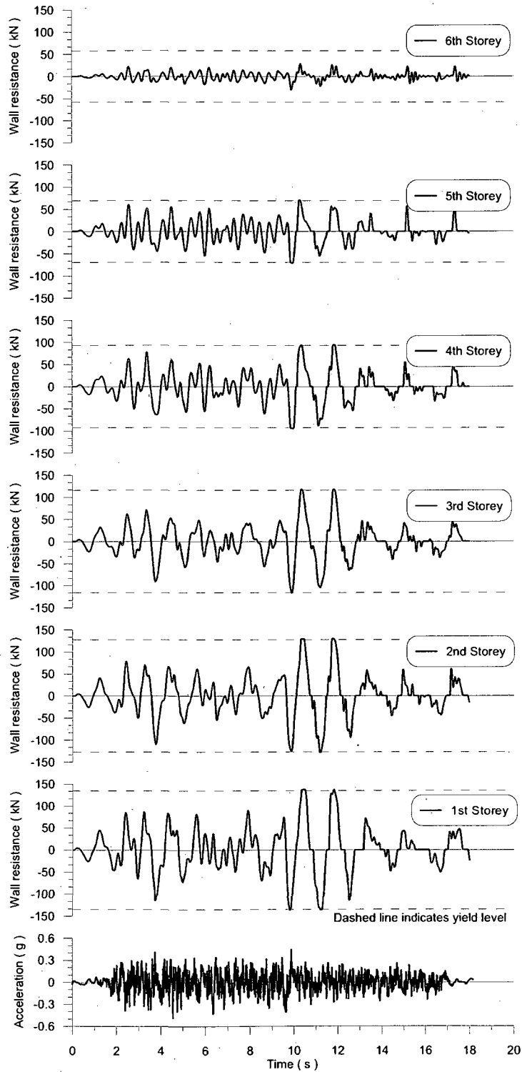
Figure H.6: Time history showing resistance vs. time for each storey, CM earthquake record,
