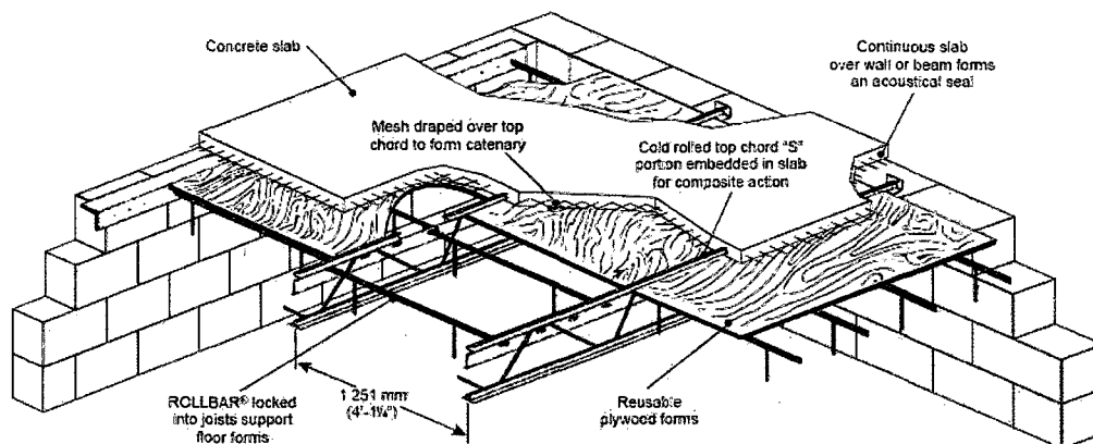
Figure 3.3: Hambro® D500 floor system ( Canam Group, 2004 )
