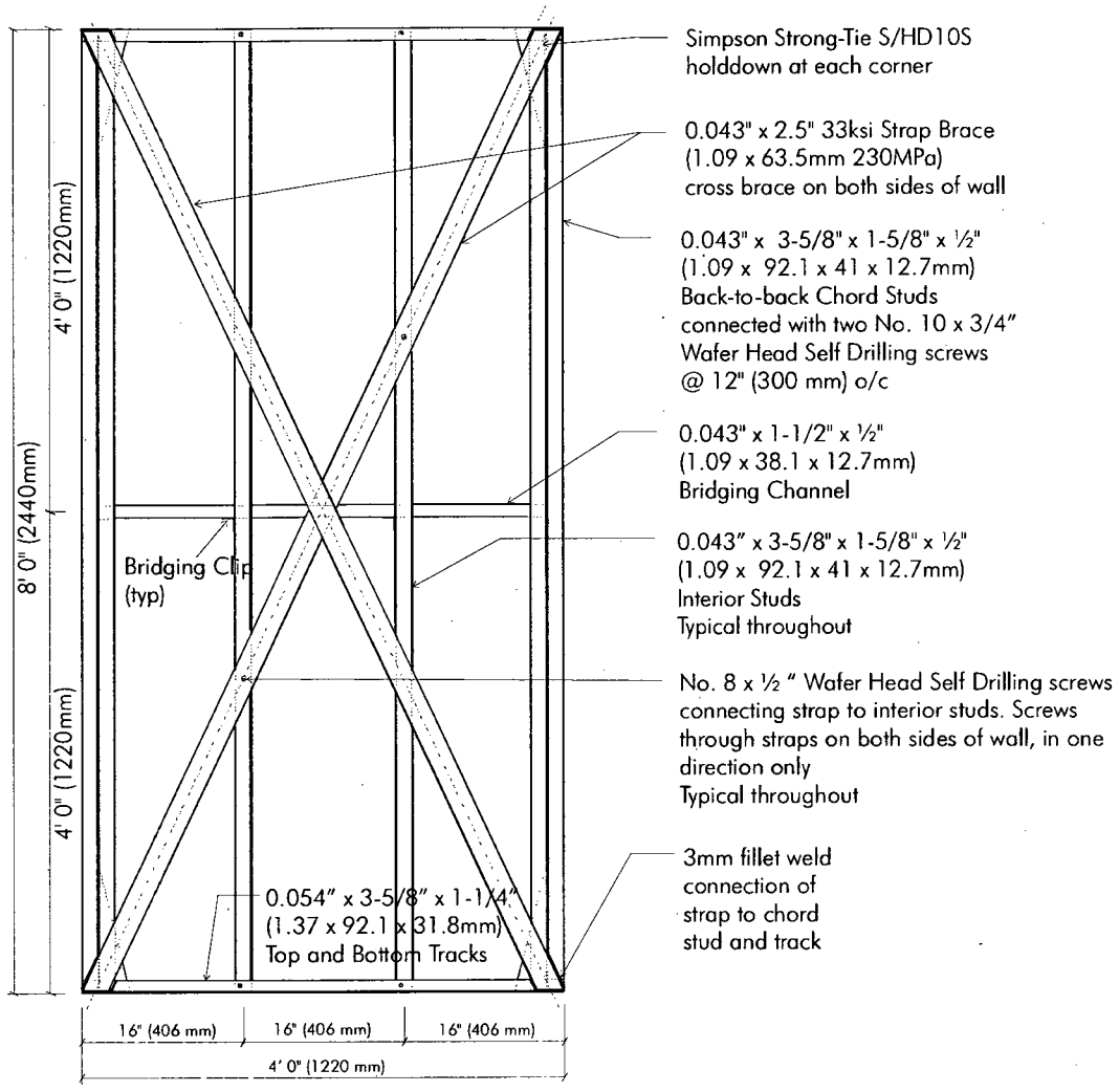
Figure B.33: Nominal dimensions and specifications for walls 15B-M and 16B-C
