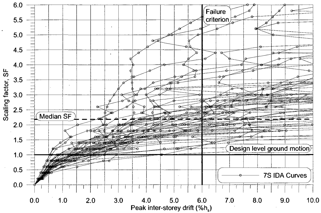
Figure I.17: IDA analysis for model 7S R_d R_o 2.6-2brace
