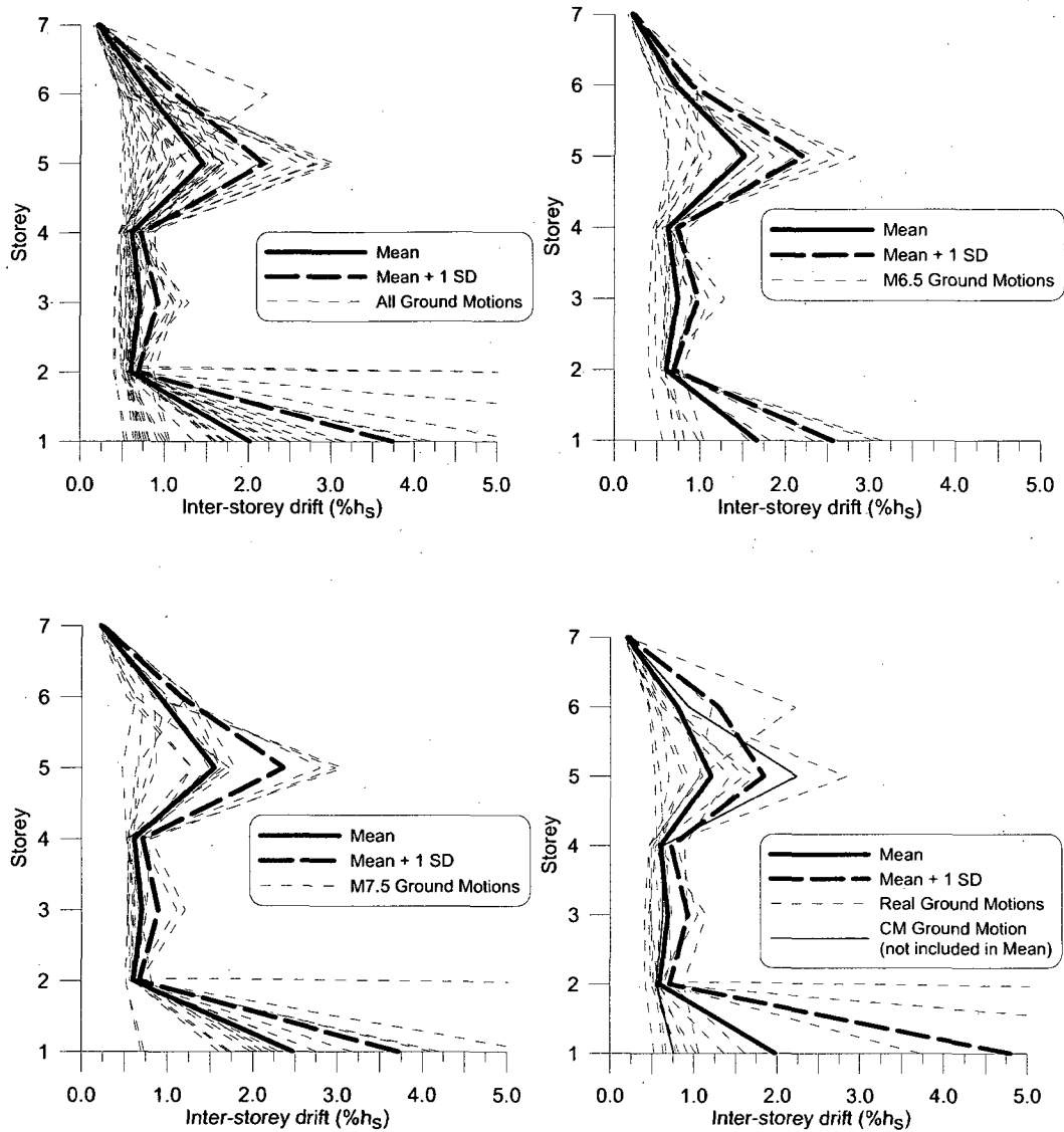
Figure I.8: Storey height versus inter-storey drift for 7S RaR04-minbrace model
