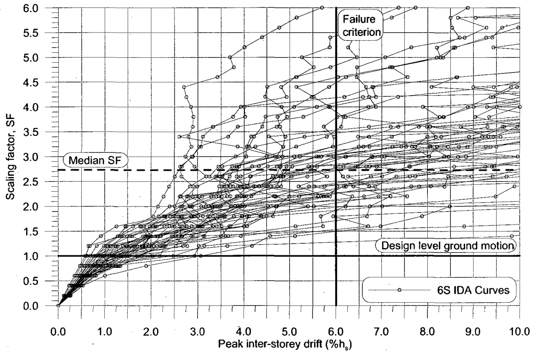
Figure I.9: IDA analysis for model 6S R_d R_o 2.6 -minbrace
