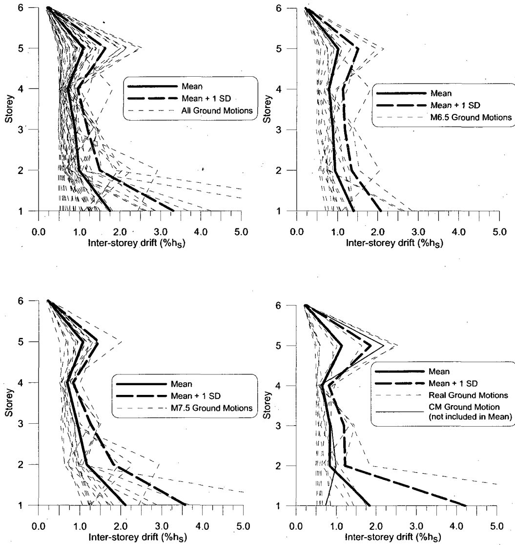
Figure I.5: Storey height versus inter-storey drift for 6S R 4 R 0 4-minbrace model
