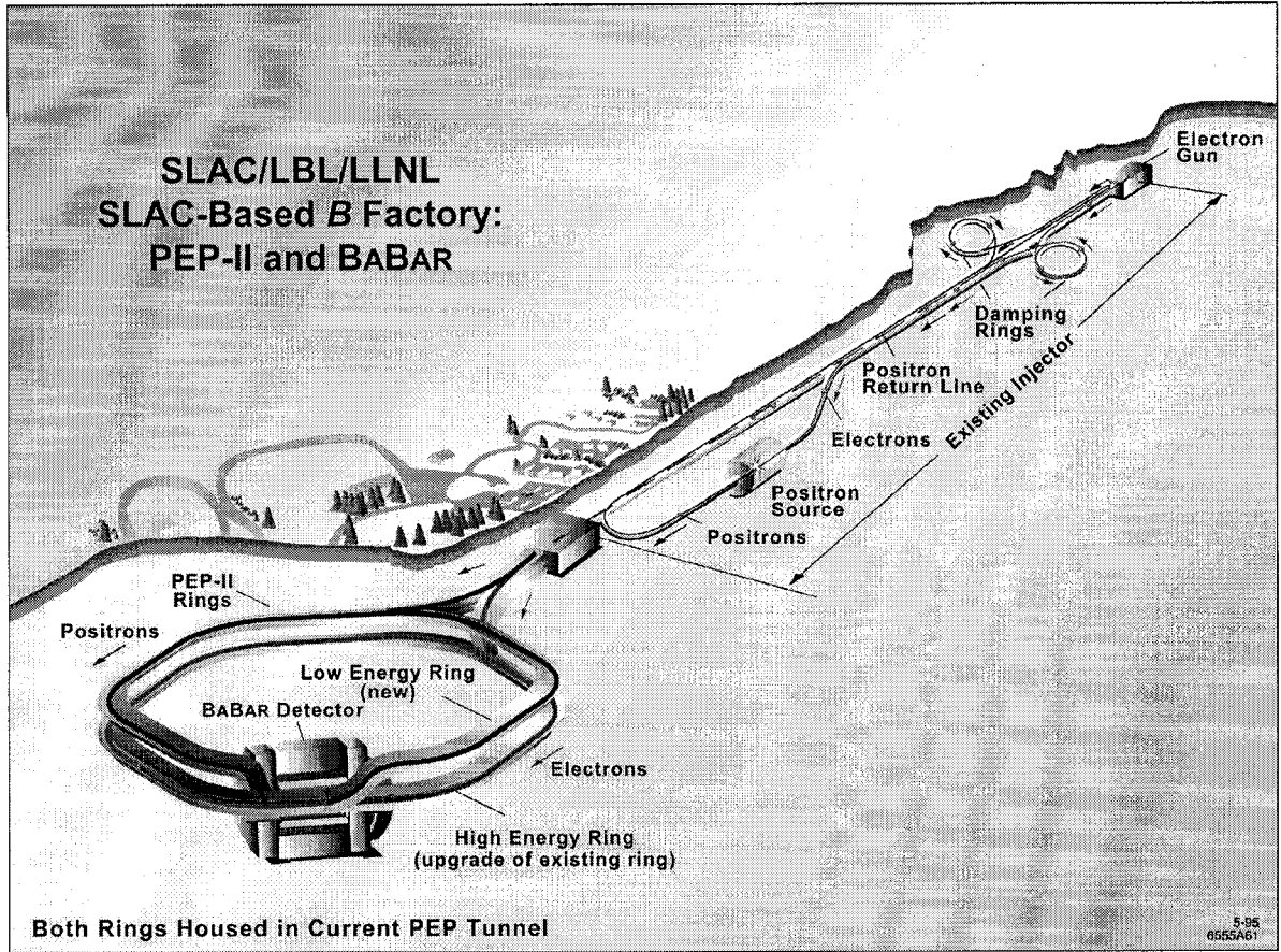
Figure 3.3: SLAC and PEP-II layout.
