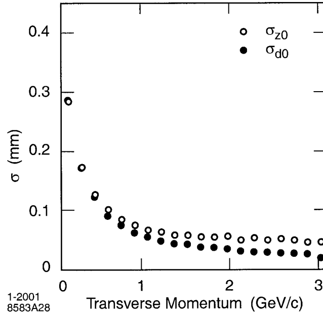
Figure 4.4: Resolutions of track parameters d_0 and z_0 as a function of transverse momentum, measured in multi-hadron events. The data are corrected for the effects of particle decays and vertexing errors. The error bars are smaller than the points shown.
