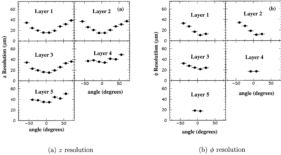
Figure 3.8: SVT hit resolution in the a) z and b) \phi coordinate in microns as a function of track incident angle. There are fewer points in the \phi resolution plots for the outer two layers because the range of incident angles subtended is much smaller.
