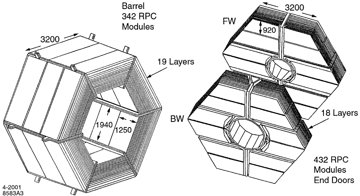
Figure 3.18: Schematic view of the IFR showing the barrel sectors and the forward(FW) and backward(BW) end doors. The shape and dimensions of the RPC modules are indicated.
