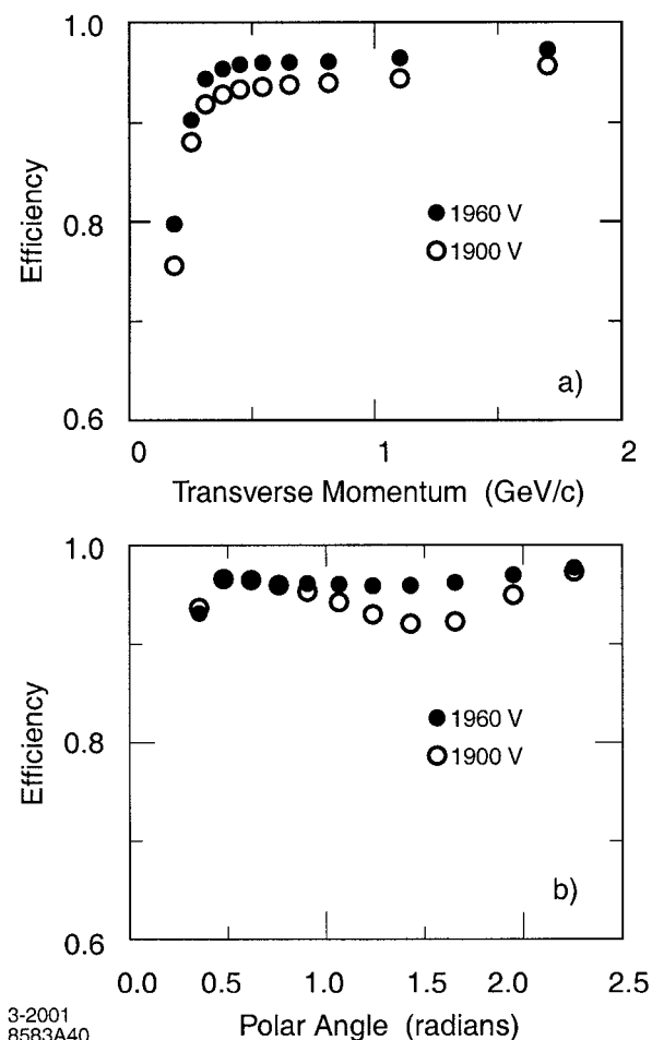
Figure 4.1: Track reconstruction efficiency in the DCH at operating voltages of 1900 V and 1960 V, as a function of a) transverse momentum, and b) polar angle. The efficiency is measured from multi-hadron events as a fraction of all tracks detected in the SVT for which the DCH portion is also reconstructed. The error bars are smaller than the points shown.
