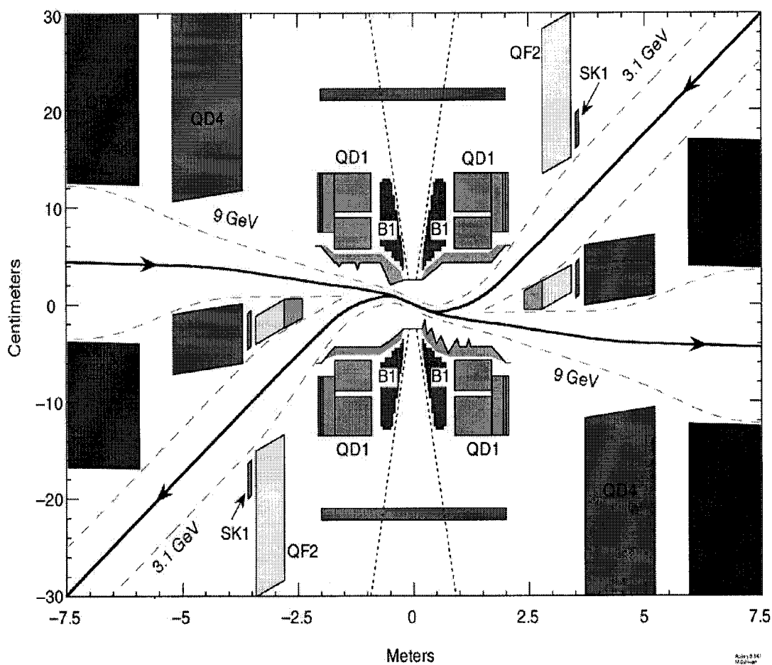
Figure 3.4: The BABAR interaction region. Shown are the final bending magnets (B1), focusing magnets, synchrotron radiation masks, and the HER/LER beam trajectories. Note the aspect ratio of the figure is not 1:1.
