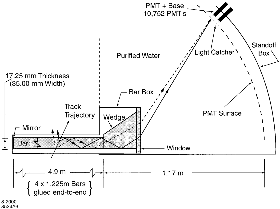
Figure 3.13: Schematics of the DIRC fused silica bar and imaging region.
