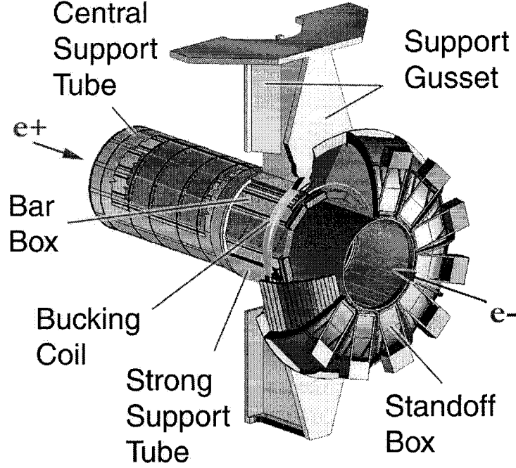
Figure 3.14: View of DIRC system.
