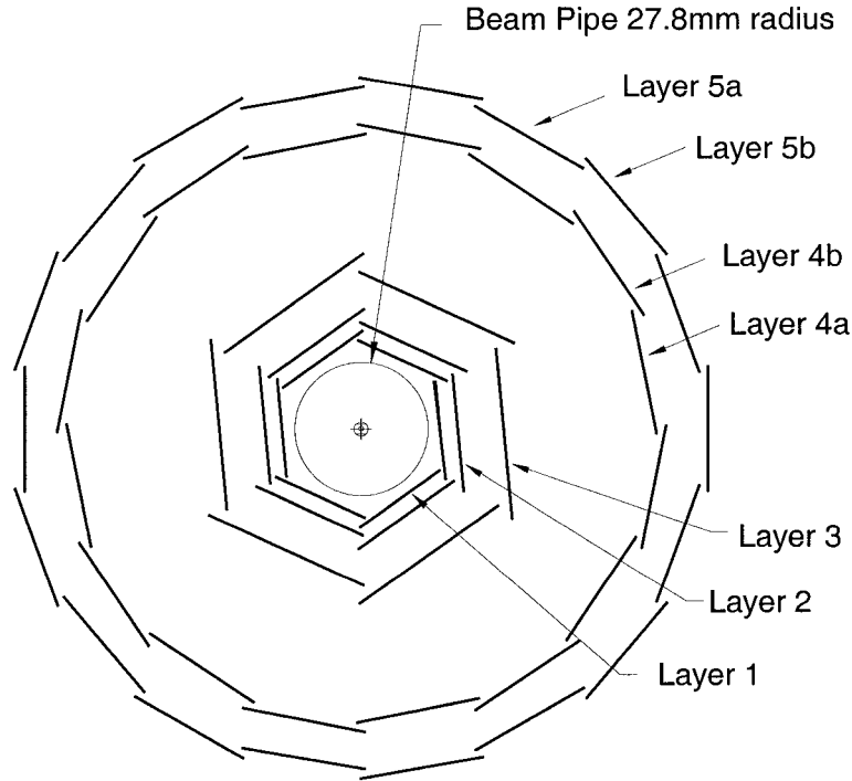
Figure 3.6: Schematic end view of the SVT.
