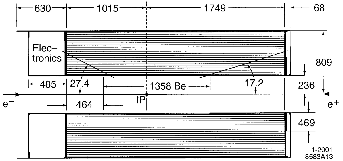
Figure 3.9: Schematic view of DCH with principle dimensions.
