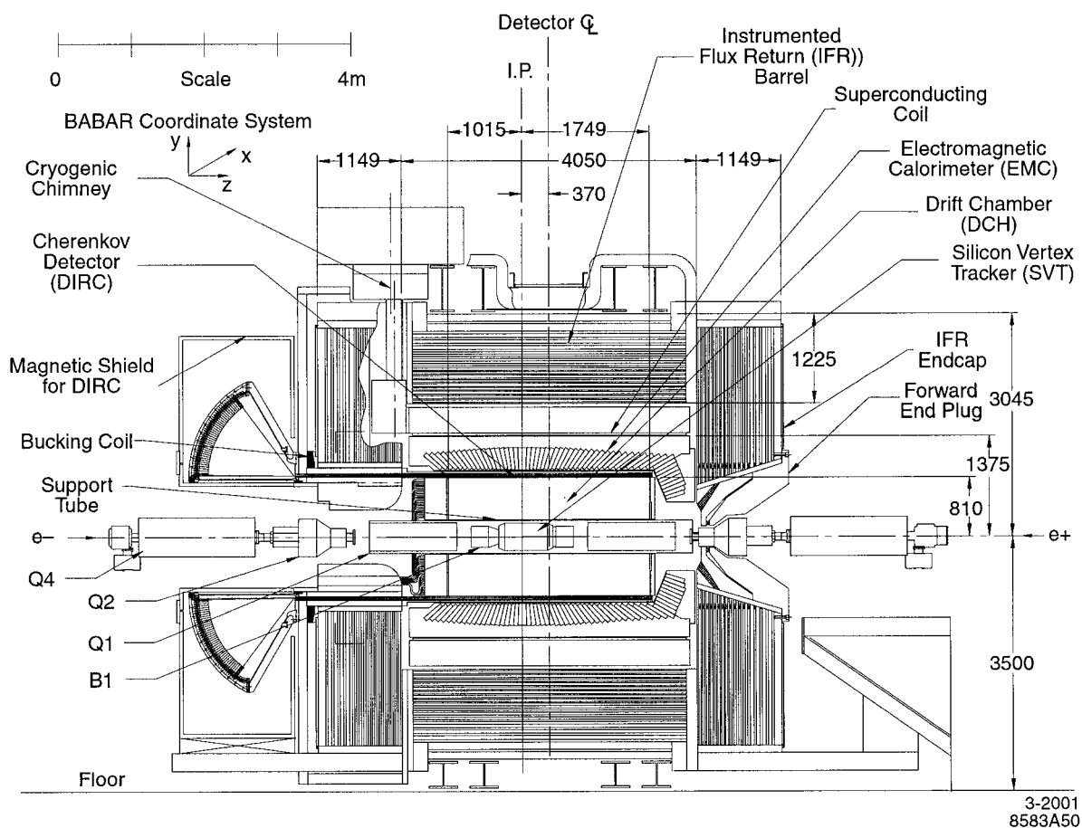
Figure 3.1: BABAR detector side view.
