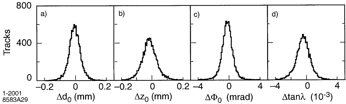
Figure 4.3: Track parameter resolutions based on the differences between the two halves of cosmic ray muon tracks with momenta above 3 GeV/c.
