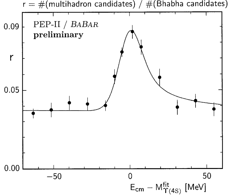
Figure 3.5: \Upsilon(4S) energy scan showing the ratio of multi-hadron events to Bhabha events.
