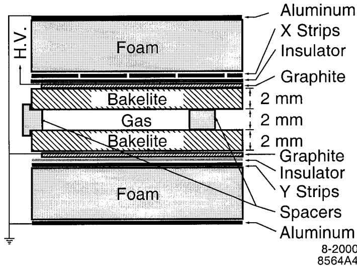
Figure 3.19: Cross section of a planar RPC with the schematics of the high voltage (HV) connection.
