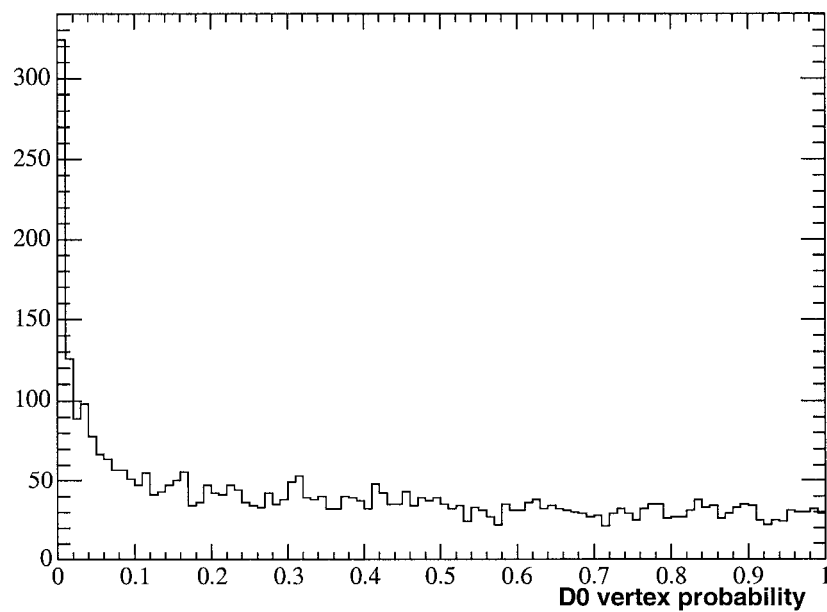
Figure 5.3: \chi^2 probability of D^0 mass-constrained fit taken from data. The cut at 0.001 is at too small a value to show on the plot.
