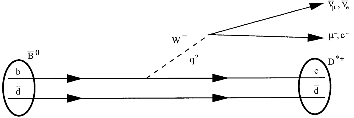
Figure 1.1: Feynman diagram of the \bar{B}^0 \rightarrow D^{*+} \ell^- \bar{\nu}_\ell decay. The virtual W boson carries 4-momentum q .
