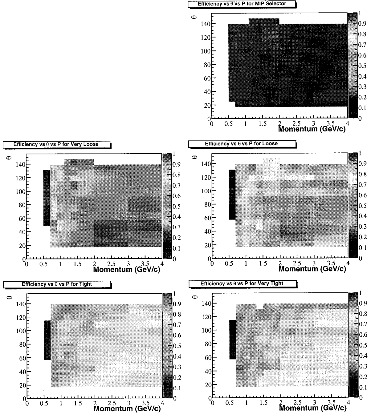
Figure A.3: \mu ID efficiencies for each selector calculated from the \mu\mu\gamma sample.
