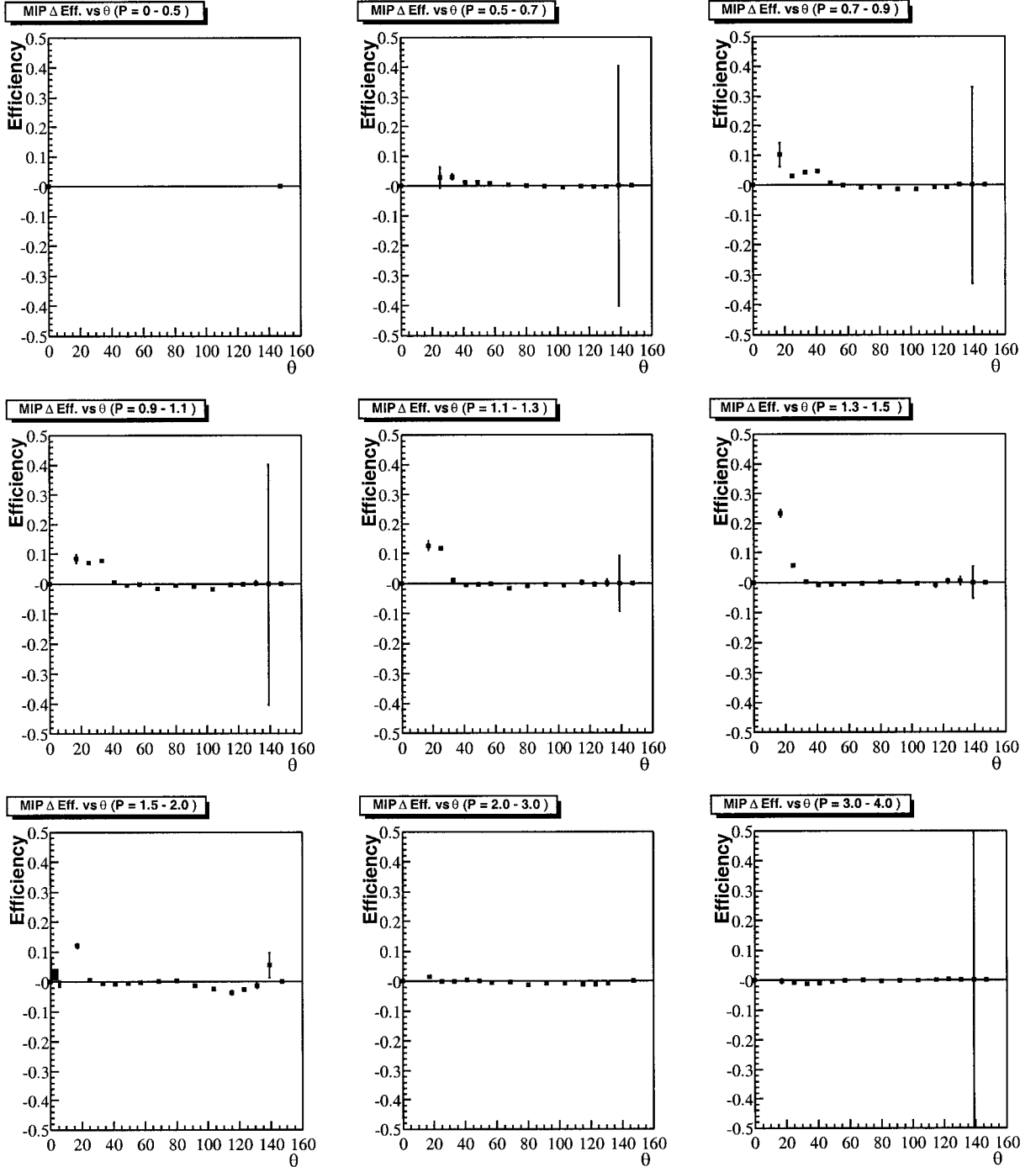
Figure A.6: Absolute efficiency differences ( \mu\mu\gamma - ee\mu\mu ) for MIP selector.
