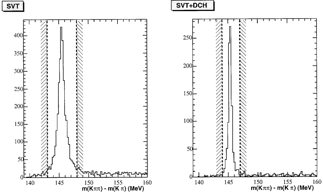
Figure 5.5: \delta m for slow pion in SVT or SVT+DCH, both taken from data. Cuts are dependent upon whether or not the slow pion enters the DCH.
