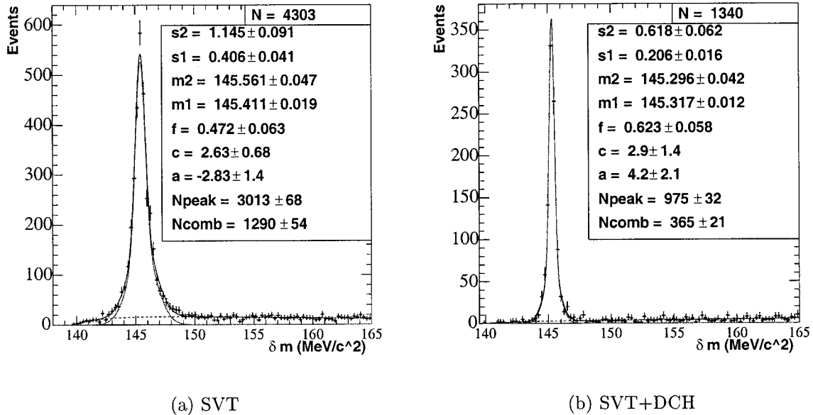
Figure 6.9: Fits to \delta m distribution for peak signal and combinatoric background from on peak data. It has been split into samples depending on whether the slow pion remains in the SVT or enters the DCH. The combinatoric background comes from events in the peaking region below the dashed line.
