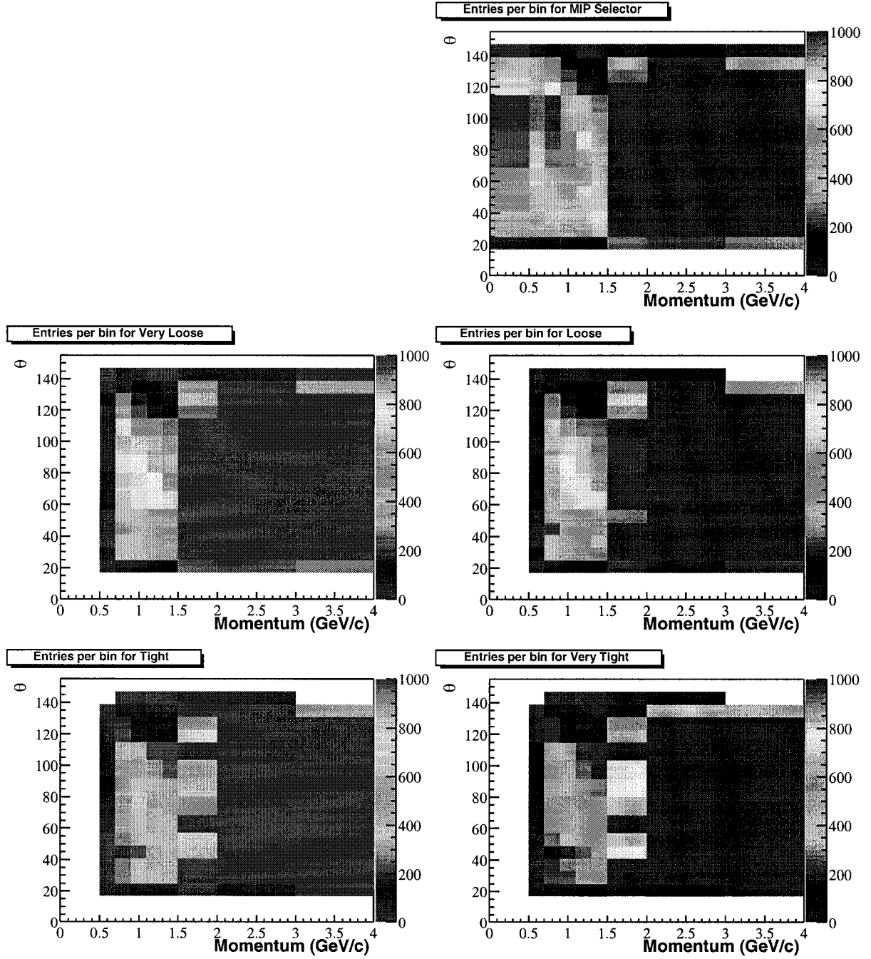
Figure A.5: Number of entries per bin in the \mu\mu\gamma sample. Bins showing maximum counts could have more than 1000 entries.
