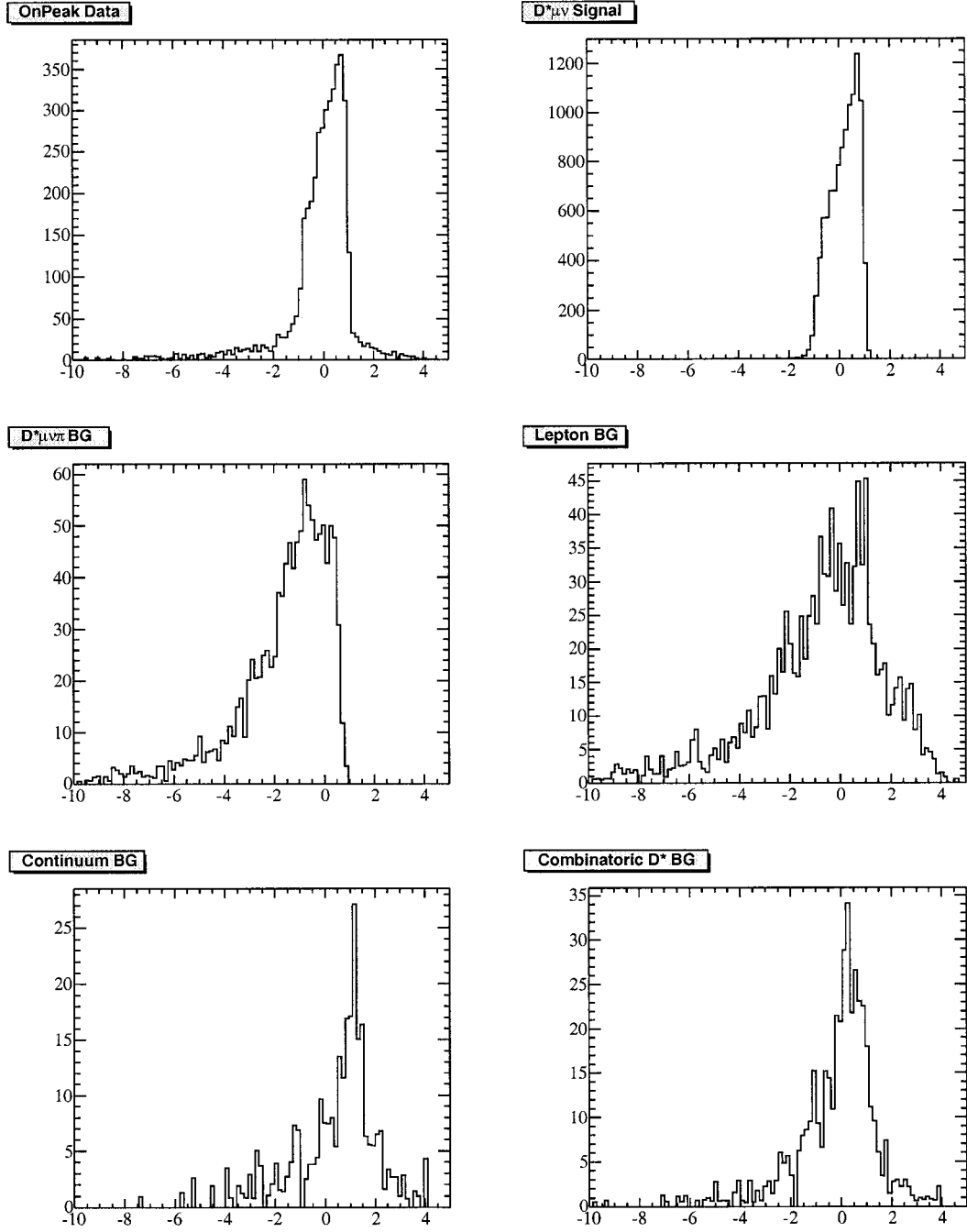
Figure 7.2: \cos \theta_{B,D^* \ell} distributions for on-peak data, \bar{B}^0 \rightarrow D^{*+} \mu^- \bar{\nu}_\mu signal, and the four background templates. These six histograms make up the inputs to the fit. Each histogram is normalized at the start of the fitting routine, so the relative number of events in each template only affects the statistical uncertainties in each bin.
