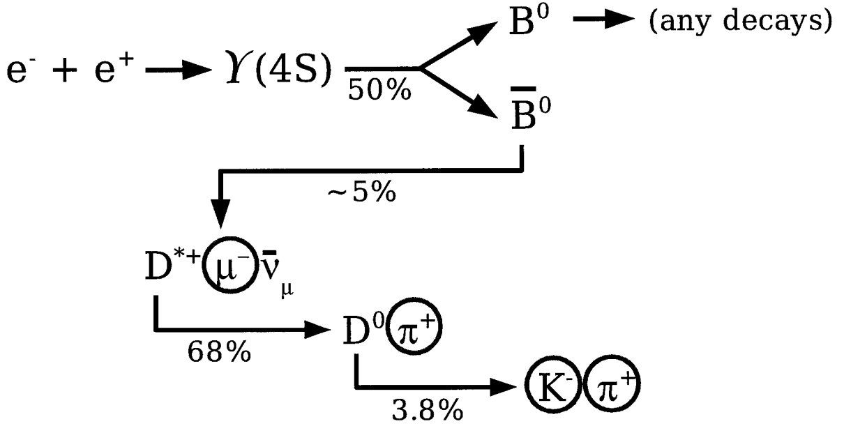
Figure 1.2: Diagram of the particle interactions involved in this analysis. At each interaction, there are numerous possible outcomes. The approximate branching fractions for the decays shown are given along the arrows. The circled particles indicate the final state particles observed by the BABAR detector. The decay of the other B meson in the event also produces detectable particles which contribute to the backgrounds in the analysis.
