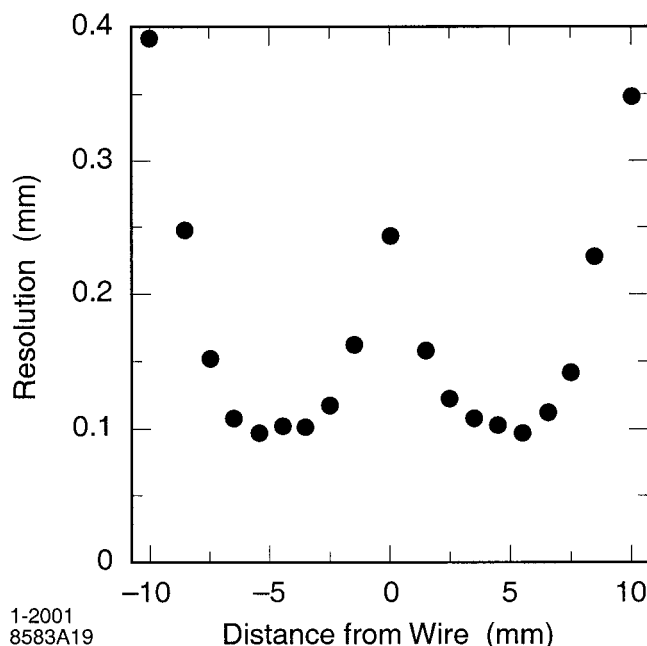
Figure 3.11: DCH position resolution vs. drift distance. Data are taken from layer 18 and averaged over all cells in the layer. Error bars are smaller than the points shown.
