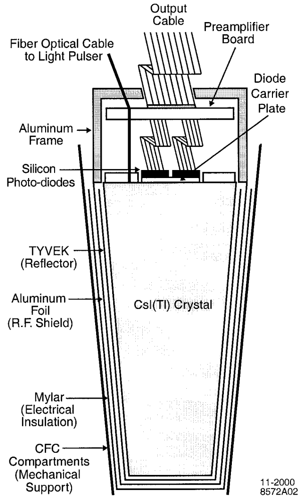
Figure 3.16: Diagram of a CsI(Tl) crystal with wrapping and readout electronics. This drawing is not to scale.
