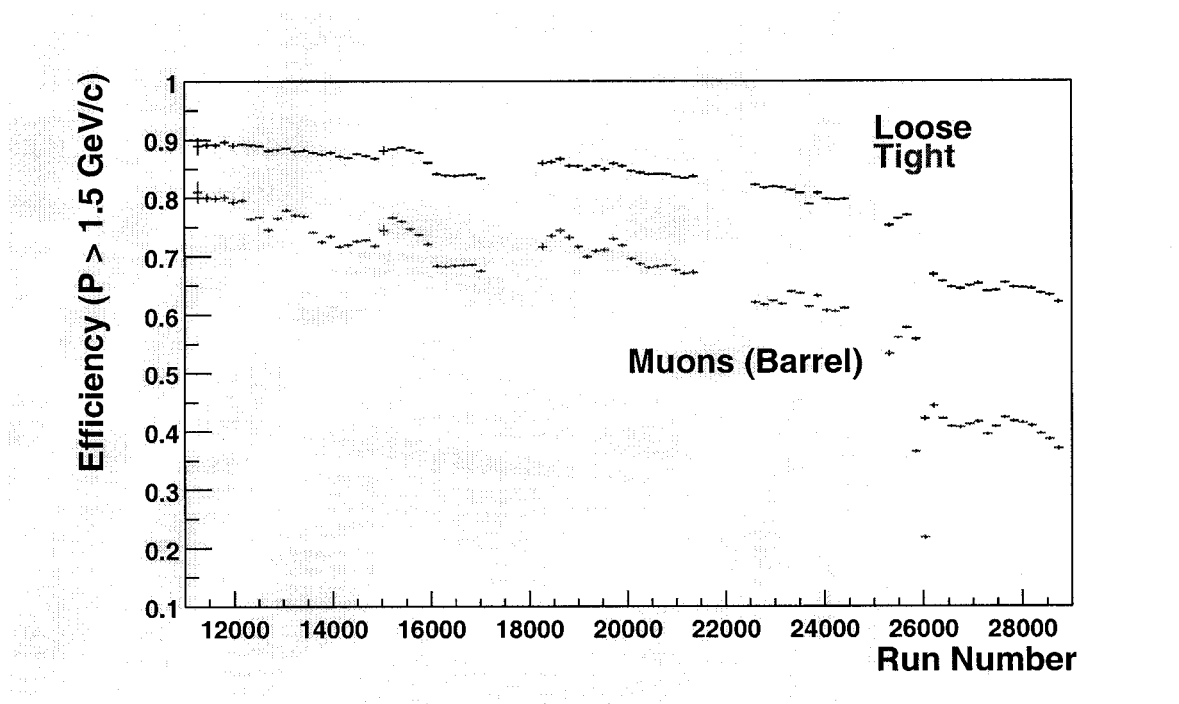
Figure 3.20: Muon detection efficiency vs. run number for data collected from 1999-2002. [34] Runs in the the 1999/2000 run period are numbered approximately 10,000 to 17,000. The labels Loose and Tight refer to the muon identification algorithms described in Section 4.2.1. The Tight mode (lower line) shows a worse decline, and is more important to this analysis. Around run number 26,000 there was a temporary failure in the IFR front-end electronics.
