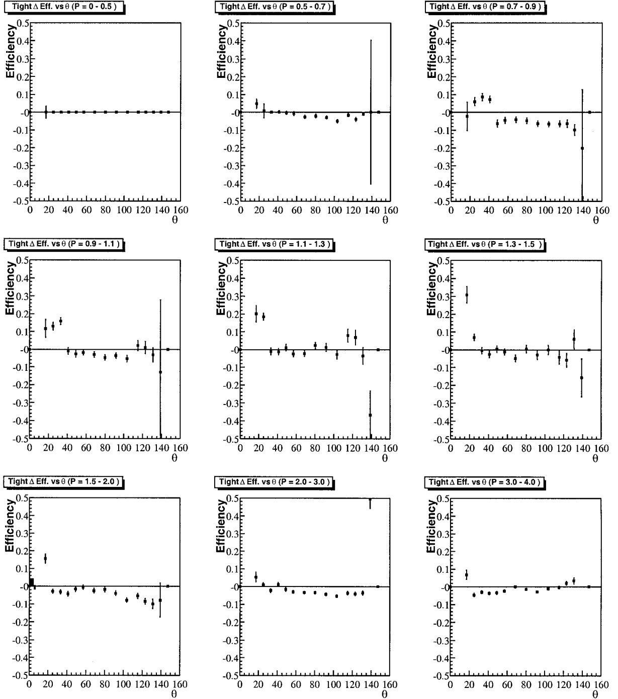
Figure A.9: Absolute efficiency differences ( \mu\mu\gamma - ee\mu\mu ) for Tight selector.
