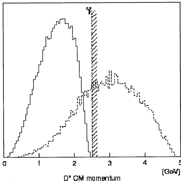
Figure 5.4: D^{*+} momentum spectra in the CM frame for signal events (solid line) and continuum events (dashed line), both taken from MC. This plot and Figure 5.7 are taken from reference 44, and the image quality is poor in the original document.
