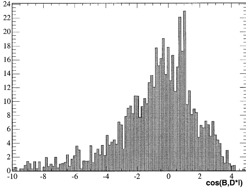
Figure 7.1: \cos\theta_{B,D^*\ell} for combined muon backgrounds taken from generic B^0 and B^\pm MC truth.
