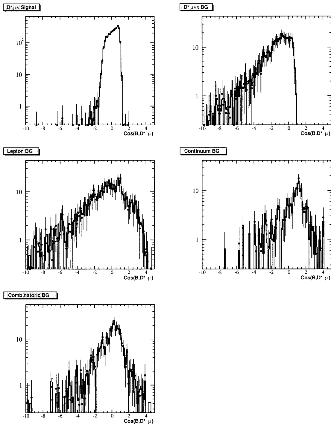
Figure 7.4: Comparing the predicted templates (line) with the input (points) for the five MC histograms used in the TFractionFitter function. The adjustments made for the predicted templates are almost always less than \frac{1}{2}\sigma for the statistical fluctuations of the bins.
