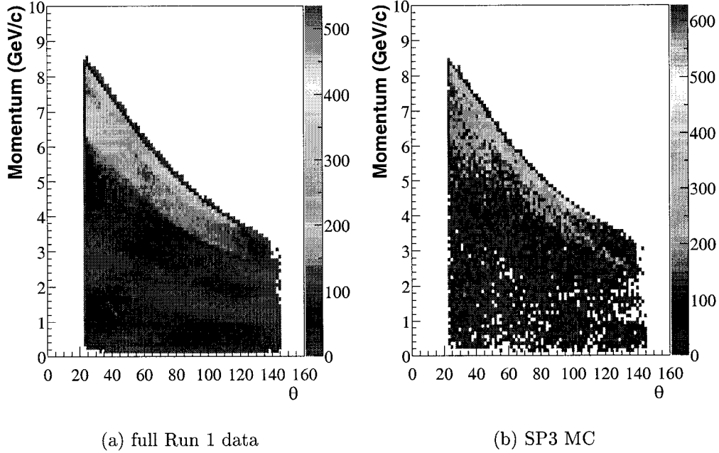
Figure A.1: Momentum vs \theta of unbiased muon tracks from data and MC.
