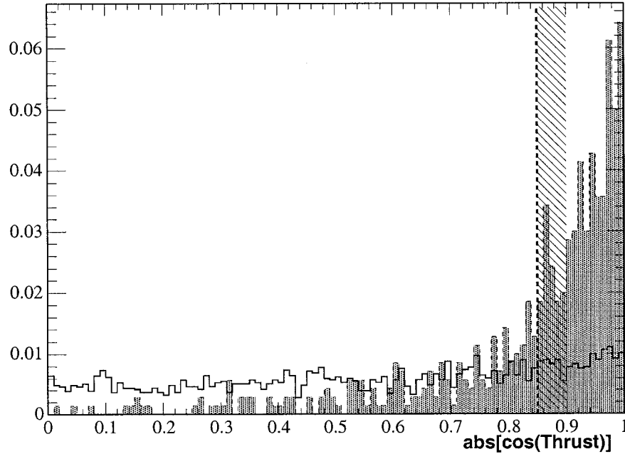
Figure 5.9: Distribution of \cos\theta_{thrust} between D^{*+}\ell^- candidate and the rest of the event for signal MC events (open histogram) and continuum background (shaded histogram) from generic charm MC.
