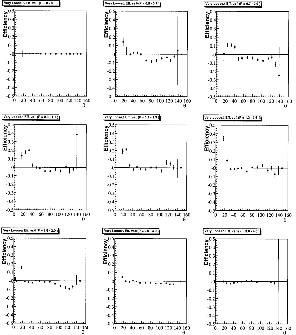
Figure A.7: Absolute efficiency differences ( \mu\mu\gamma - ee\mu\mu ) for Very Loose selector.
