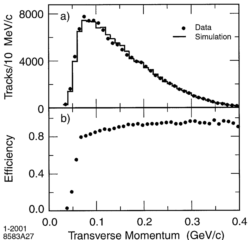
Figure 4.2: Monte Carlo studies of low momentum tracks in the SVT: a) comparison of data (contributions from combinatoric background and non- B\bar{B} events have been subtracted) with simulation of the transverse momentum spectrum of pions from D^{*+} \rightarrow D^0\pi^+ in B\bar{B} events, and b) efficiency for slow pion detection derived from simulated events.
