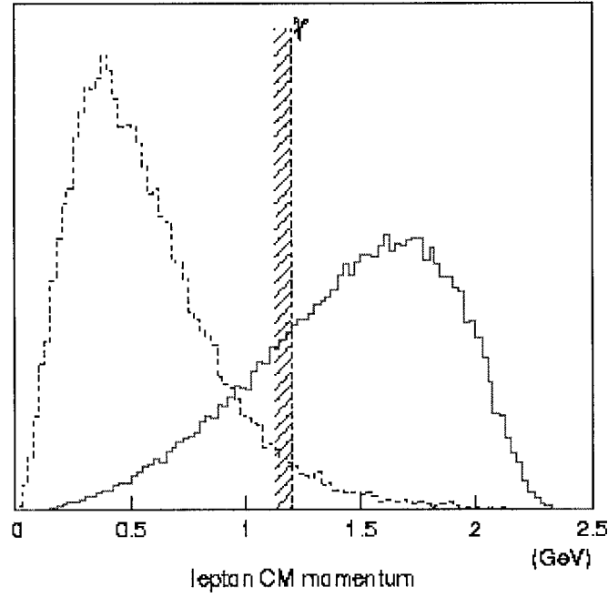
Figure 5.7: Lepton momentum spectrum in CM frame for signal (solid line) and background (dashed line) leptons from generic B MC. [44]
