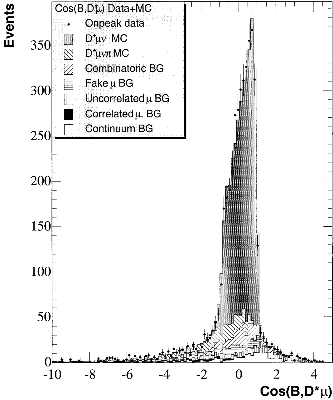
Figure 7.3: Fit Results. The data points are overlaid on the sum of the MC template histograms. The templates shown are the predicted templates after the fit has completed, scaled by the fractions returned by the fit. The three muon backgrounds are taken from the individual histograms before they were merged for the fit, but all are scaled by the muon background fraction.
