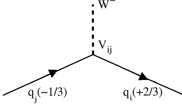
Figure 2.1: Feynman diagram of a quark of charge -1/3 decaying into a +2/3 charged quark through the release of a virtual W boson.
