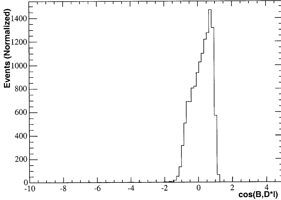
Figure 6.1: \cos\theta_{B,D^*\ell} for \bar{B}^0 \rightarrow D^{*+}\mu^-\bar{\nu}_\mu signal events from generic B^0 and \bar{B}^0 \rightarrow D^{*+}\mu^-\bar{\nu}_\mu single-mode MC truth.
