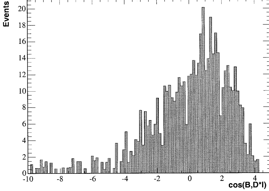
Figure 6.5: \cos \theta_{B,D^*\ell} for uncorrelated muon background taken from generic B^0 and B^\pm MC truth.
