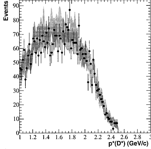
Figure 8.3: Comparisons of D^* momentum in the CM frame for data and MC. The data is shown by the points. The shaded band represents the 1\sigma contour for the generic MC.
