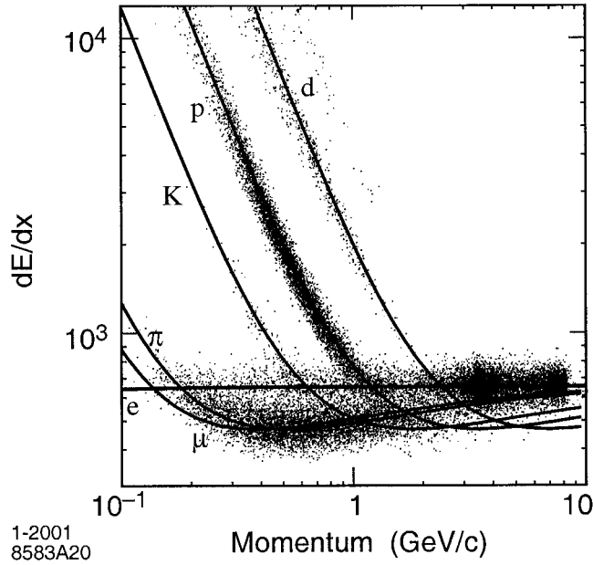
Figure 3.12: Measurements of dE/dx vs. track momenta. The data include large samples of beam background triggers, as can be seen from the high rate of protons. The superimposed curves represent Bethe-Bloch predictions for different particle species.
