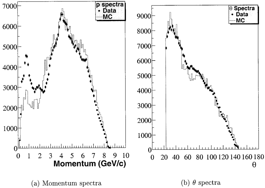
Figure A.2: Spectra of unbiased muon tracks in data and MC.
