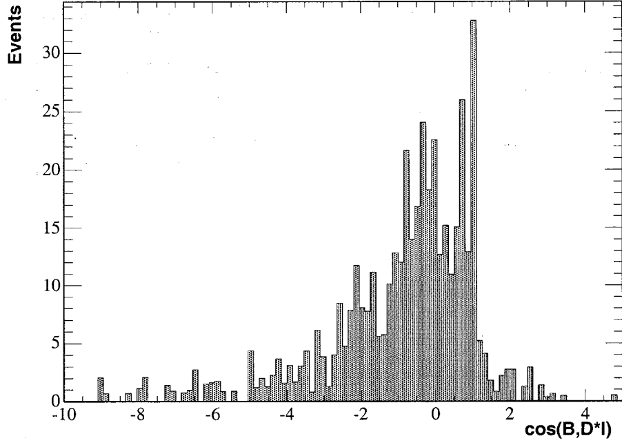
Figure 6.6: \cos \theta_{B,D^*\ell} for fake muon background taken from generic B^0 and B^\pm MC truth.
