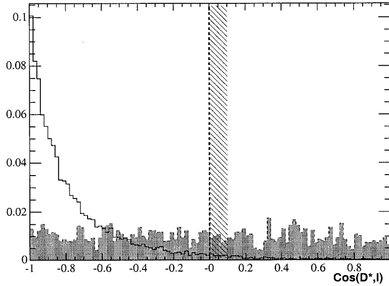
Figure 5.8: \cos \theta_{D^*, \ell} for \bar{B}^0 \rightarrow D^{*+} \ell^- \bar{\nu}_\ell signal (open histogram) and background (filled) leptons taken from generic B MC. Both histograms are normalized to unit area. In almost all of the signal events, the D^{*+} and the \ell^- are in opposite hemispheres in the CM frame.
