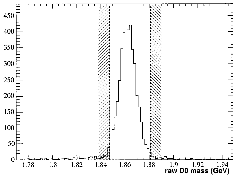
Figure 5.2: Raw D^0 candidate mass distribution taken from data. The cuts applied are shown. In this and subsequent plots, the hash marks on the cut line indicate the data removed by the cut.
