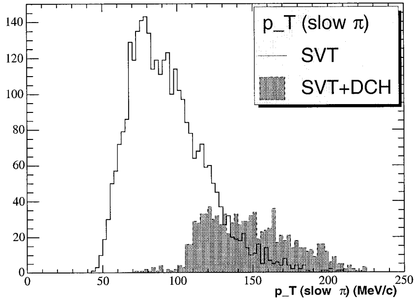
Figure 5.6: Transverse momentum of slow pion in SVT or SVT+DCH taken from data. The majority of the slow pions fail to reach the DCH.
