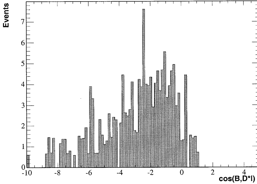
Figure 6.4: \cos \theta_{B,D^*l} for correlated muon background taken from generic B^0 and B^\pm MC truth.
