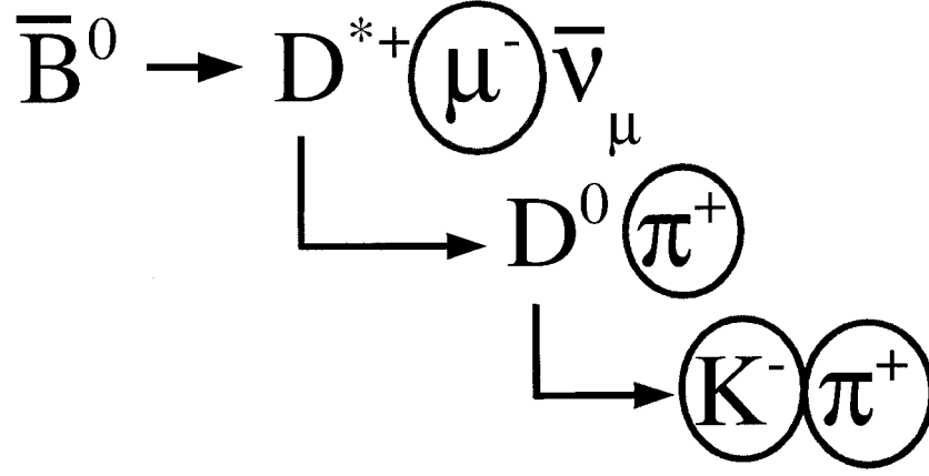
Figure 5.1: The decay chain reconstructed in this analysis. The circled particles are seen as tracks in the detector. The B and D mesons decay too quickly to leave any tracks, and neutrinos are undetectable by BABAR .
