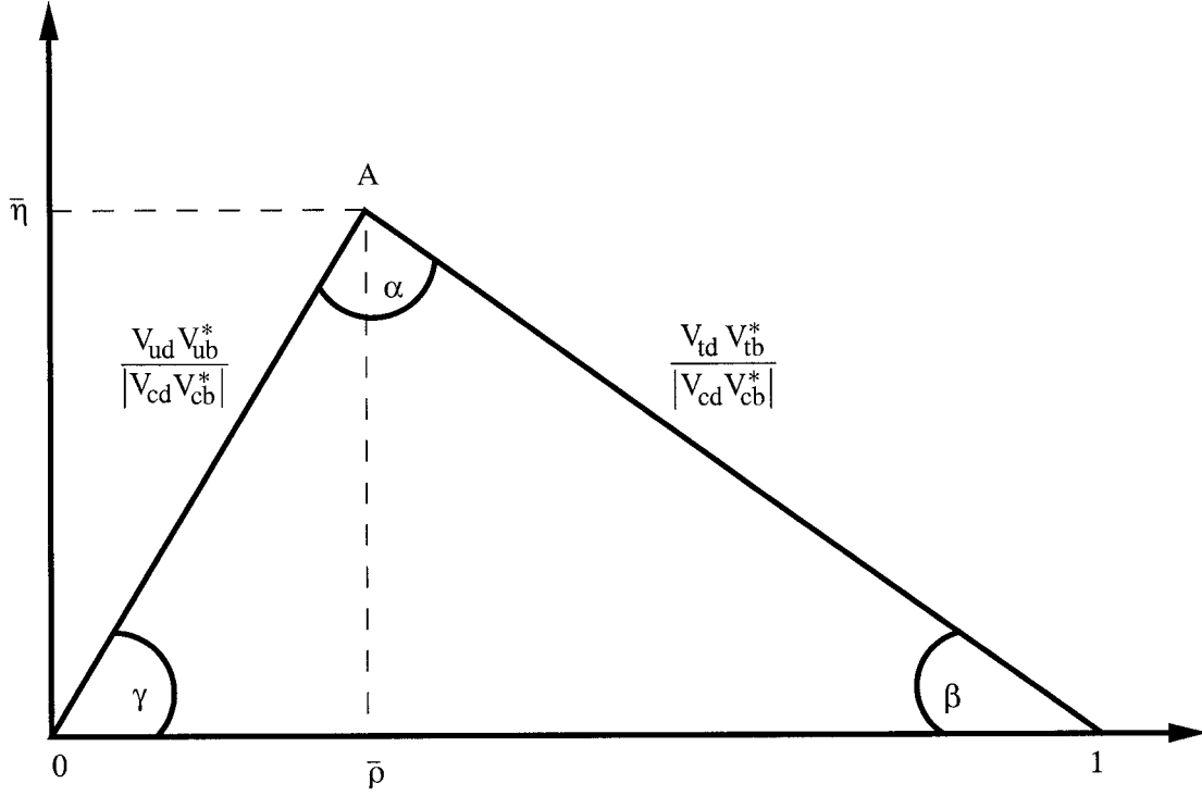
Figure 2.2: The unitarity triangle of the CKM matrix, normalized to 1 along the base. The top point of the triangle corresponds to \bar{\rho} = (1 - \lambda^2/2)\rho and \bar{\eta} = (1 - \lambda^2/2)\eta .
