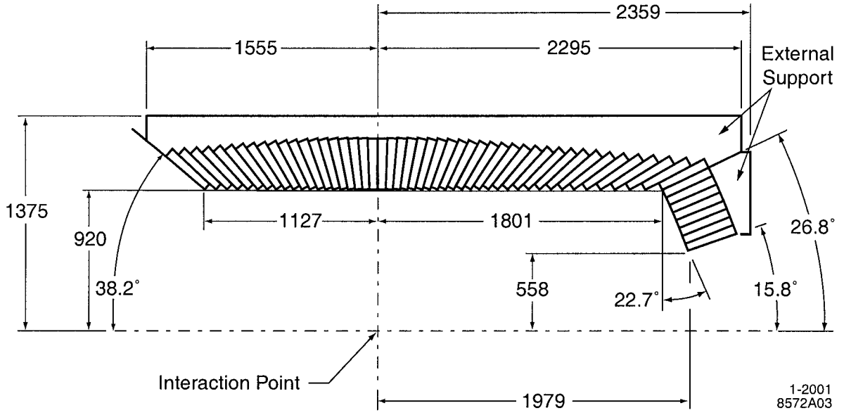
Figure 3.15: Cross sectional view of the top half of the EMC showing the arrangement of the 56 rings of CsI crystals. The detector is axially symmetric around the z -axis. All dimensions are given in mm.
