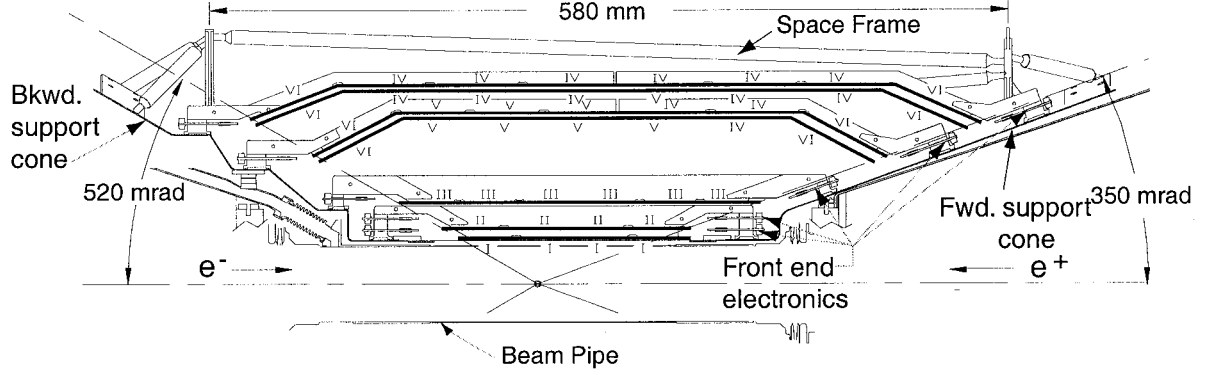
Figure 3.7: Side view of the SVT. The roman numerals represent the six different types of sensors.
