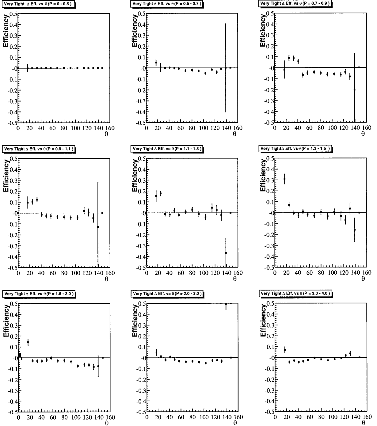
Figure A.10: Absolute efficiency differences ( \mu\mu\gamma - ee\mu\mu ) for Very Tight selector.
