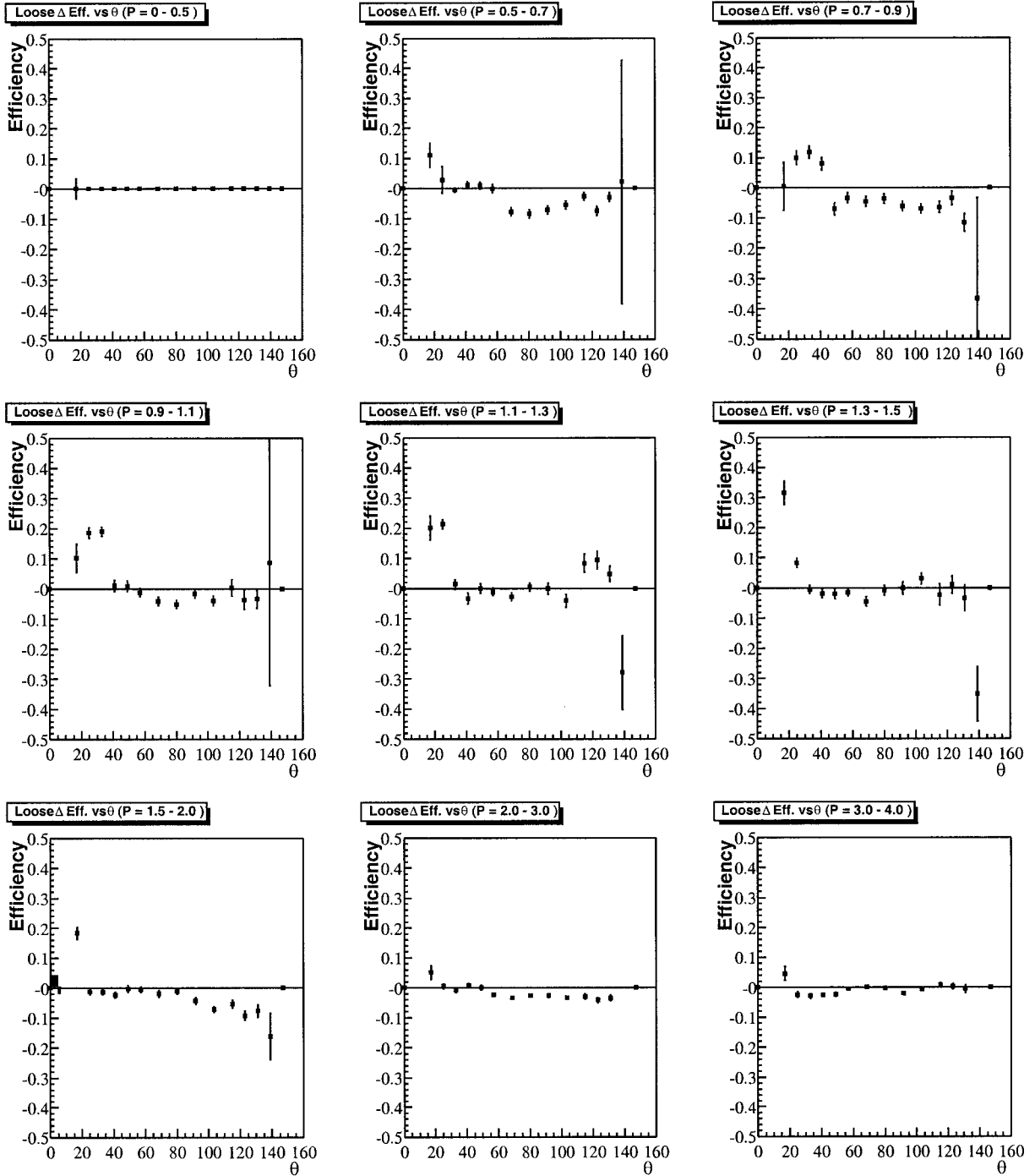
Figure A.8: Absolute efficiency differences ( \mu\mu\gamma - ee\mu\mu ) for Loose selector.
