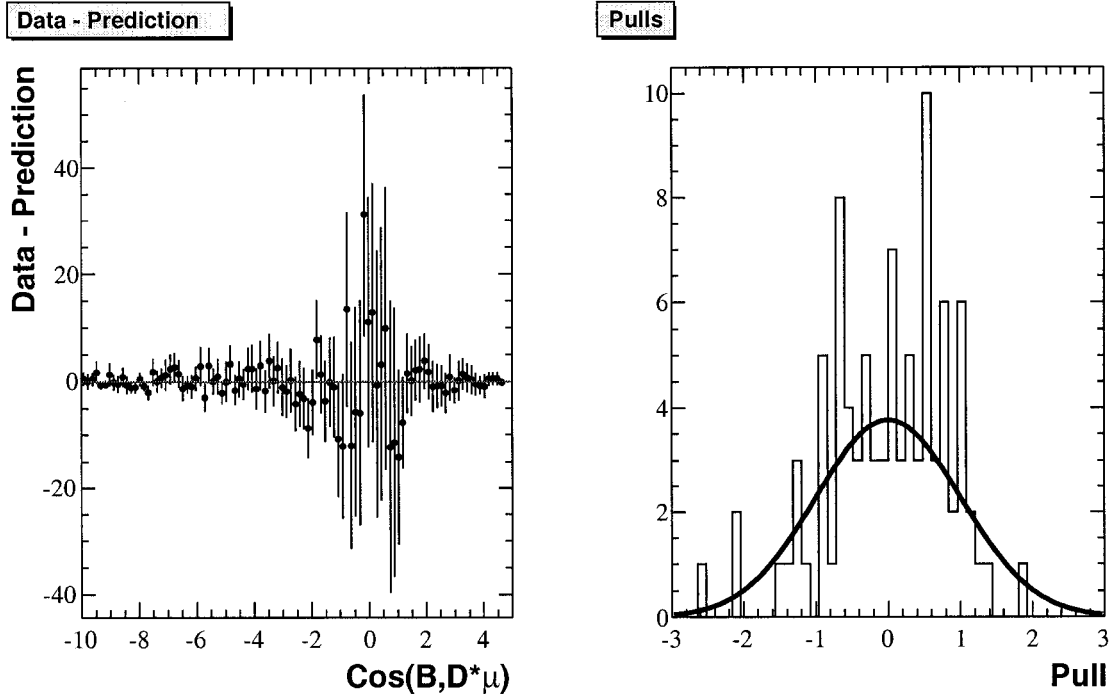
Figure 7.5: The left plot shows the difference between the data and the prediction in each bin. The pulls are shown in the right plot. A Gaussian distribution of width 1 is fit to the pulls to show an ideal result.
