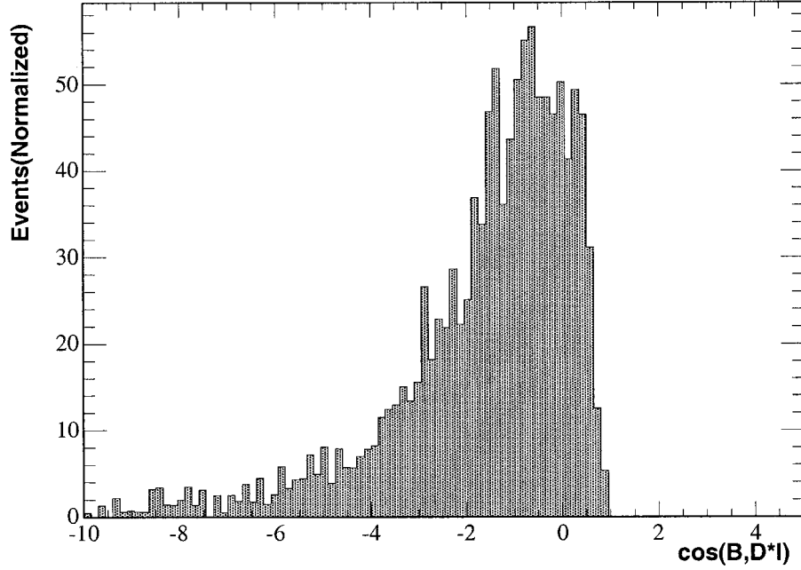
Figure 6.3: \cos \theta_{B,D^*\ell} for B \rightarrow D^{*+} \mu^- \bar{\nu}_\mu \pi background taken from generic B^0 and B^\pm MC using truth information.
