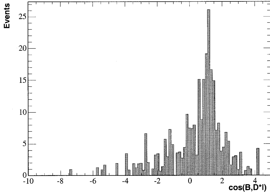
Figure 6.7: \cos \theta_{B,D^*l} for continuum background taken from generic c\bar{c} MC truth.
