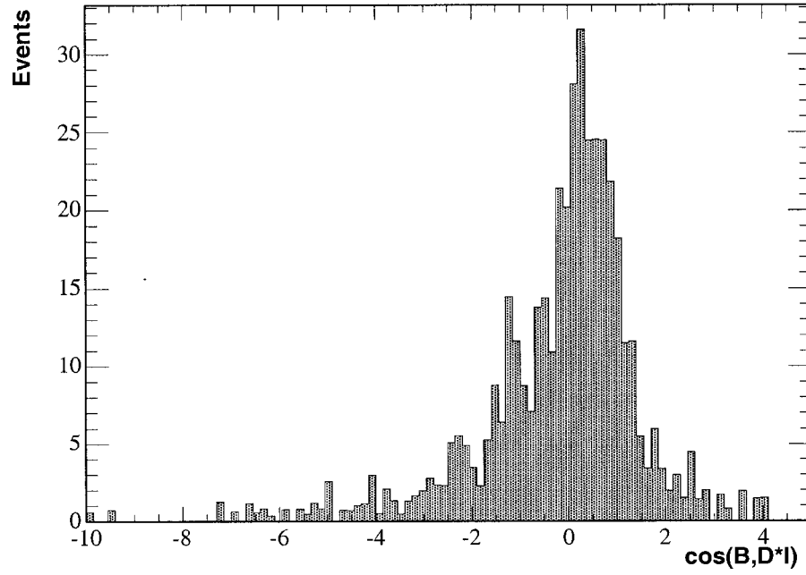
Figure 6.8: \cos \theta_{B,D^*l} for combinatoric background taken from generic B^0 and B^\pm MC truth.
