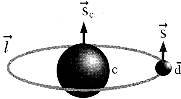
Figure 6.2: Pictorial view of the D meson.
