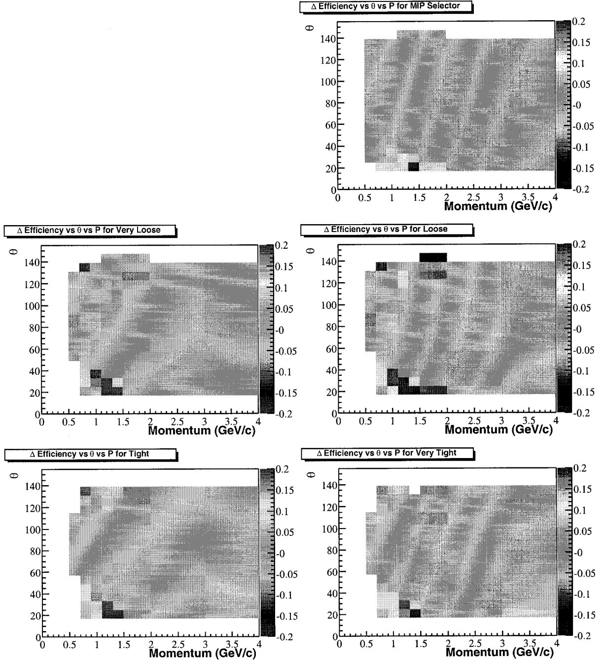
Figure A.4: Absolute efficiency differences between the \mu\mu\gamma and ee\mu\mu control samples. The values are calculated from \mu\mu\gamma - ee\mu\mu .
