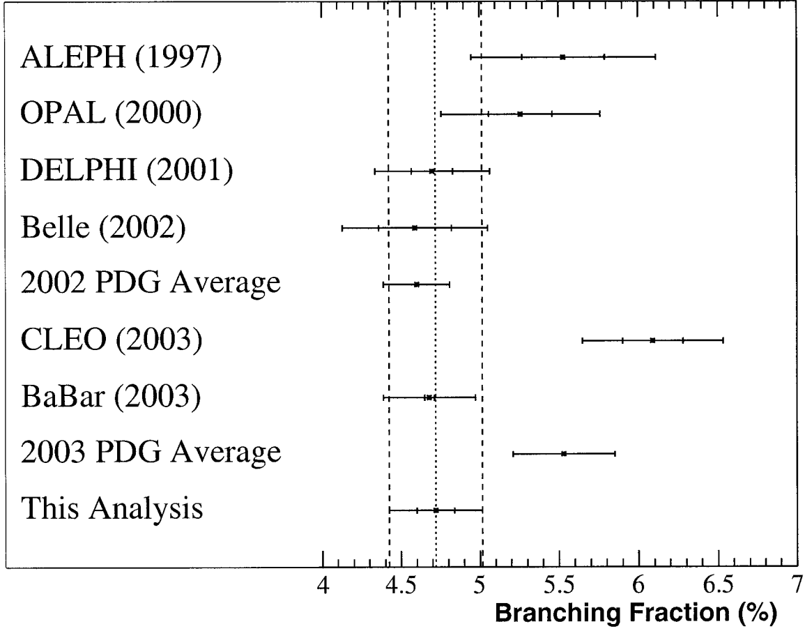
Figure 9.1: Comparison to \mathcal{B}(\bar{B}^0 \rightarrow D^{*+} \mu^- \bar{\nu}_\mu) measurements from BABAR and other experiments. This analysis shows very good agreement to the other results, with the possible exception of the CLEO measurement. [6, 7, 10, 67–71]
