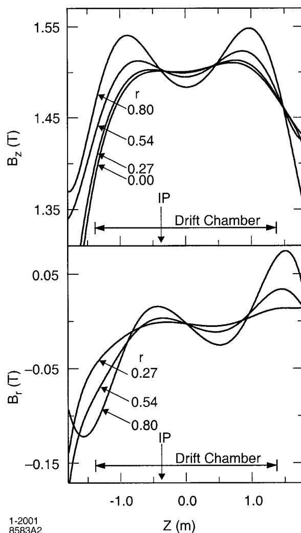
Figure 3.17: Magnetic field components B_z and B_r as a function of z . The curves represent measurements at different radial distances, r (metres). The extent of the DCH and the IP are indicated.
