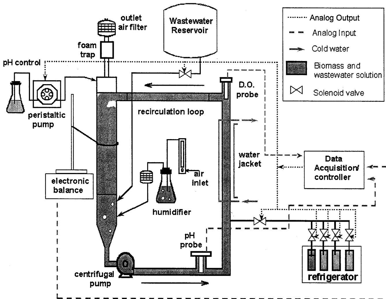
Figure 4.6: Experimental Apparatus.
