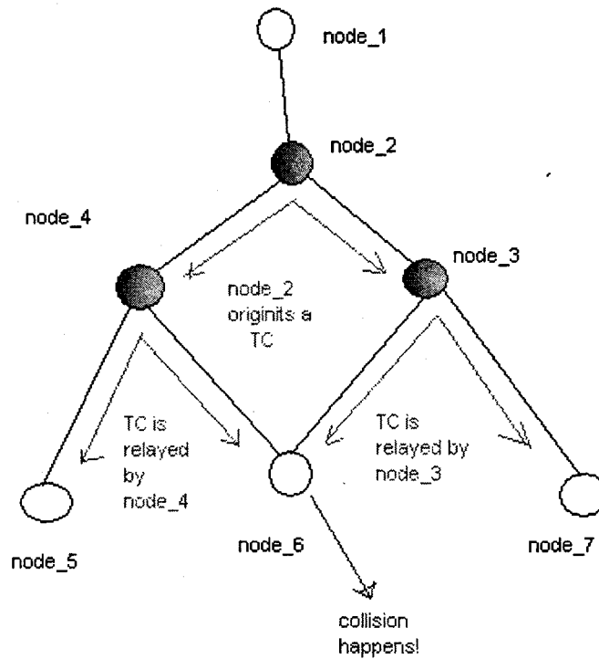
Figure 15: An Example for TC Packet Collisions at the Physical Layer
