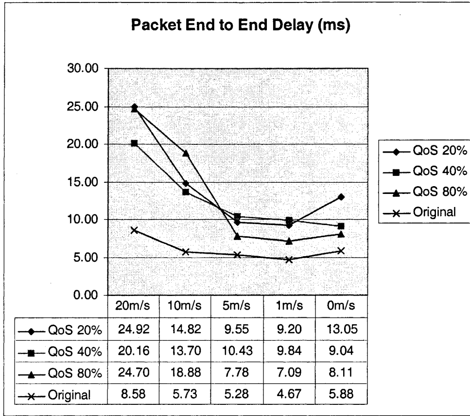
Figure 17: Comparison of End-To-End Delay of Data Packets for 4 OLSR Algorithms in 50-Nodes-Network
