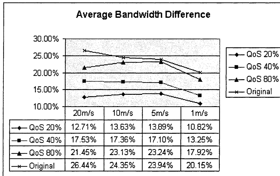
Figure 27: Comparison of Average Bandwidth Difference for 4 OLSR Algorithms in 30-Nodes-Network
