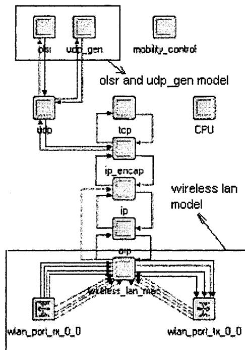
Figure 7: OLSR Node
