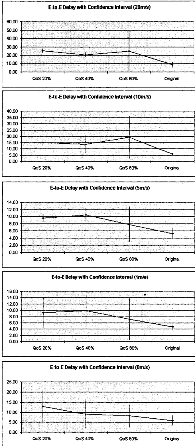
Figure 22: End-To-End Delay Comparison with Confidence Intervals
