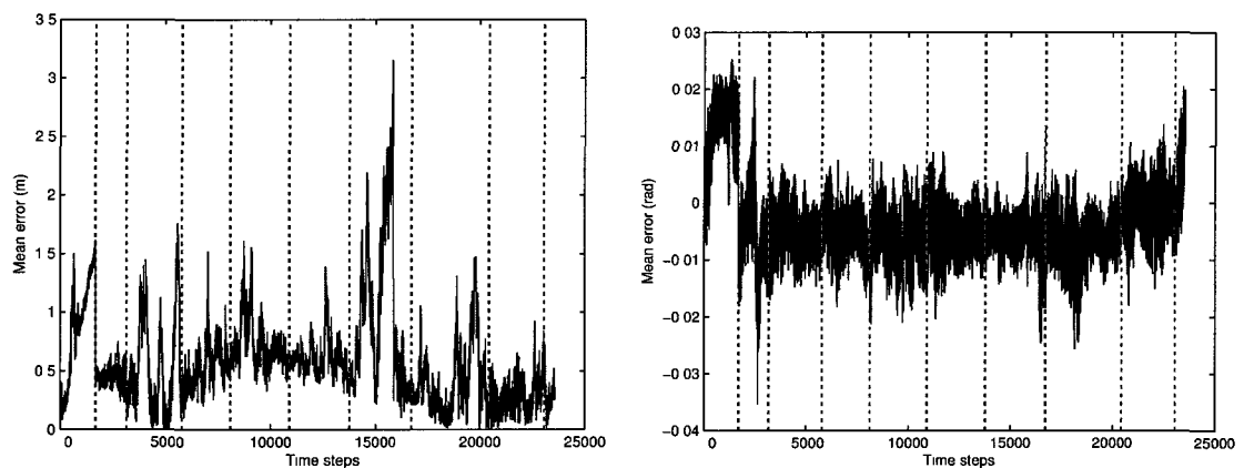
Figure 5.11: MbotSim localization global error e_1 with \mathbf{Q}_2 noise.
