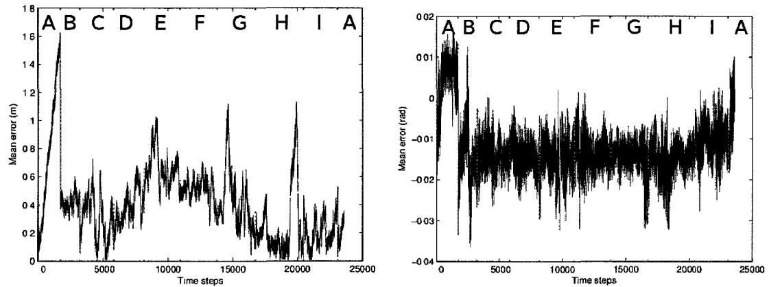
Figure 5.6: MobotSim localization global error e_1 with Q_1 noise.
