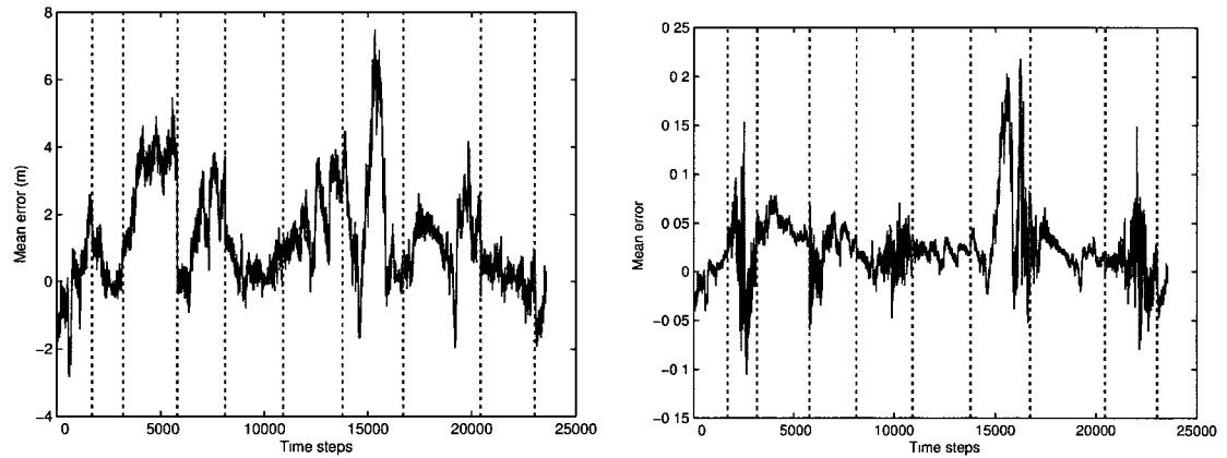
Figure 5.31: RobotSim localization node map reference error e_4 and e_5 with \mathbf{Q}_3 noise.
