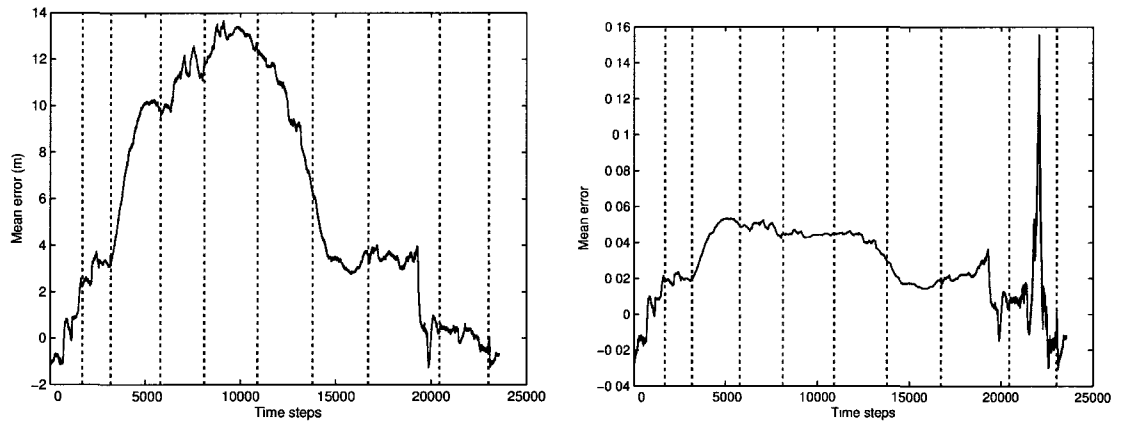
Figure 5.22: MobotSim localization global reference error e_4 and e_5 with Q_1 noise.
