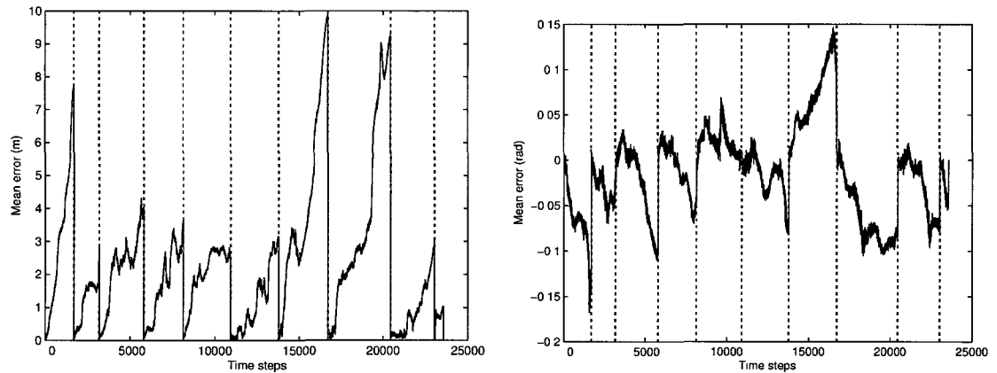
Figure 5.20: MobotSim localization node maps error e_1 with Q_1 noise.
