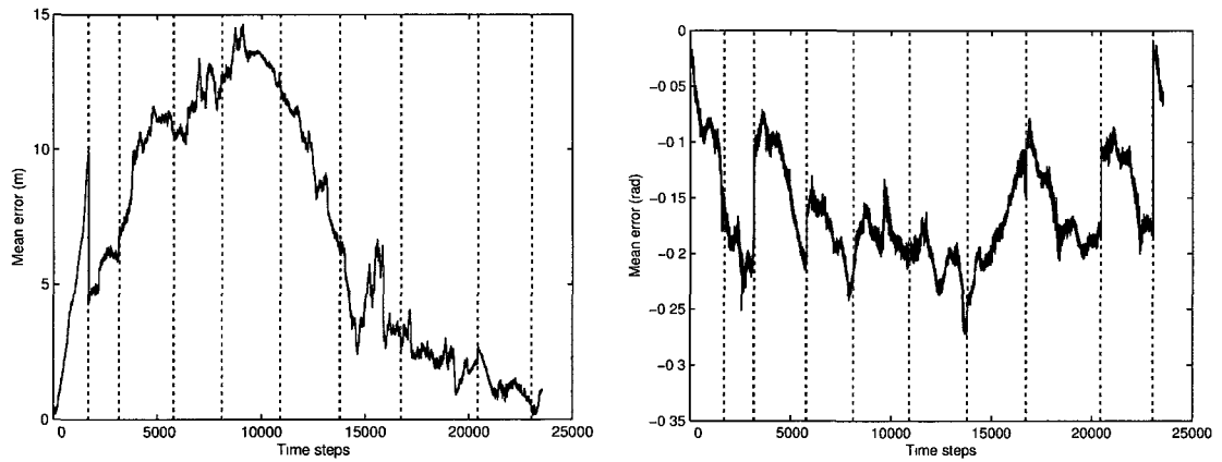
Figure 5.24: MbotSim localization global error e_1 with Q_2 noise.
