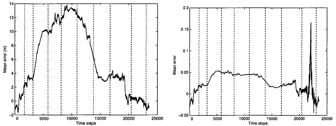
Figure 5.27: MobotSim localization global reference error e_4 and e_5 with \mathbf{Q}_2 noise.
