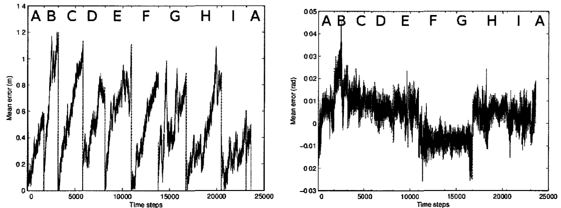
Figure 5.7: MobotSim localization node maps error e_1 with Q_1 noise.
