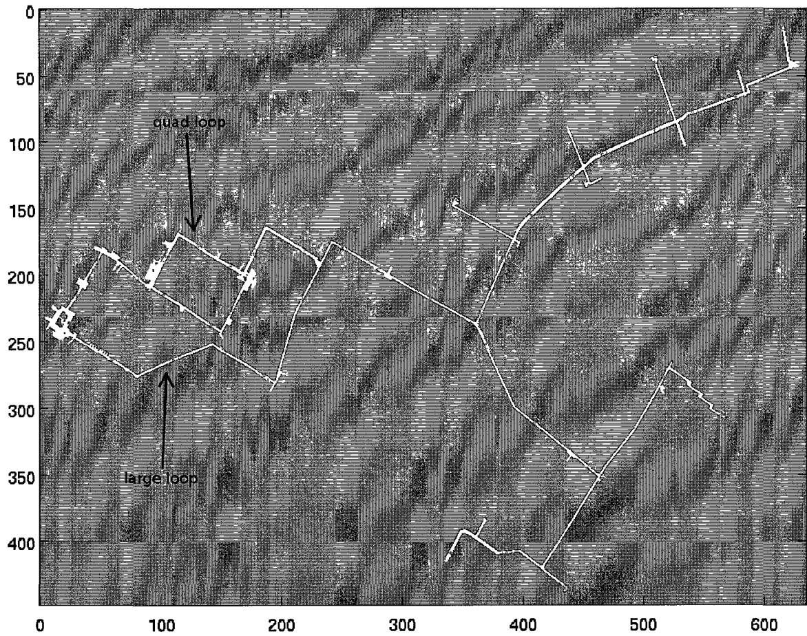
Figure 4.3: Carleton University global map with green circles marking RFID tags (metres).
