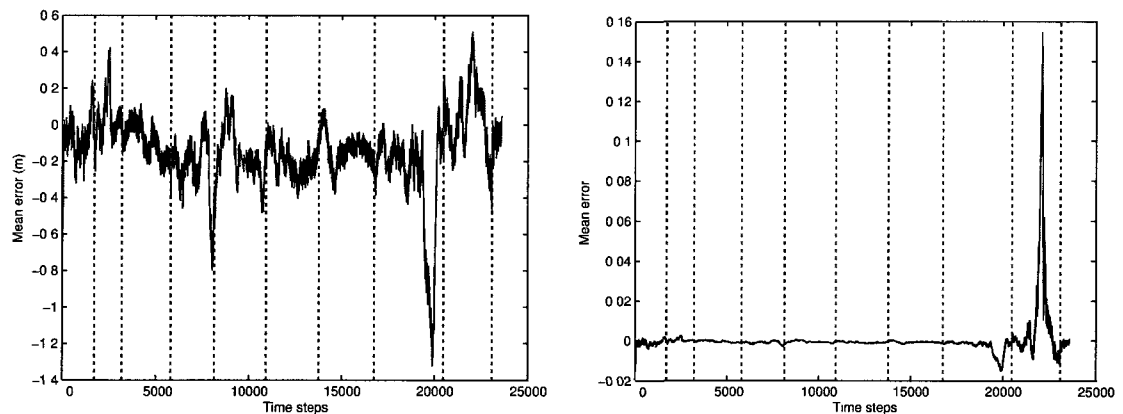
Figure 5.9: MobotSim localization global reference error e_4 and e_5 with Q_1 noise.
