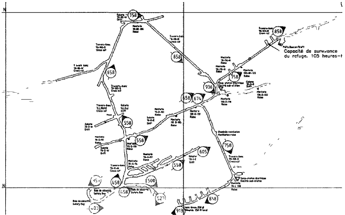
Figure 1.1: CANMET CAD Map.
