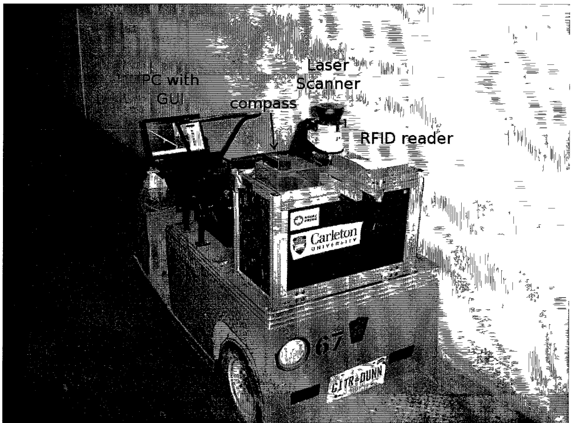
Figure 4.1: Taylor-Dunn SS-534 vehicle with sensors in the CU tunnel network.
