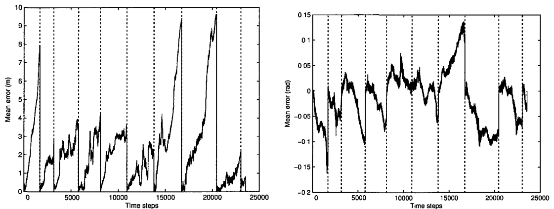
Figure 5.25: MbotSim localization node maps error e_1 with Q_2 noise.
