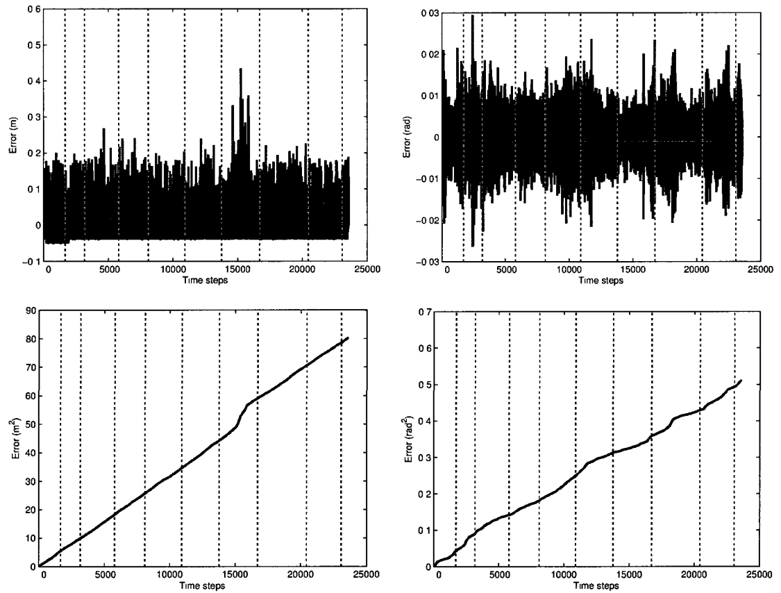
Figure 5.13: MobotSim localization error e_2 and cumulative e_2^2 with Q_2 noise.
