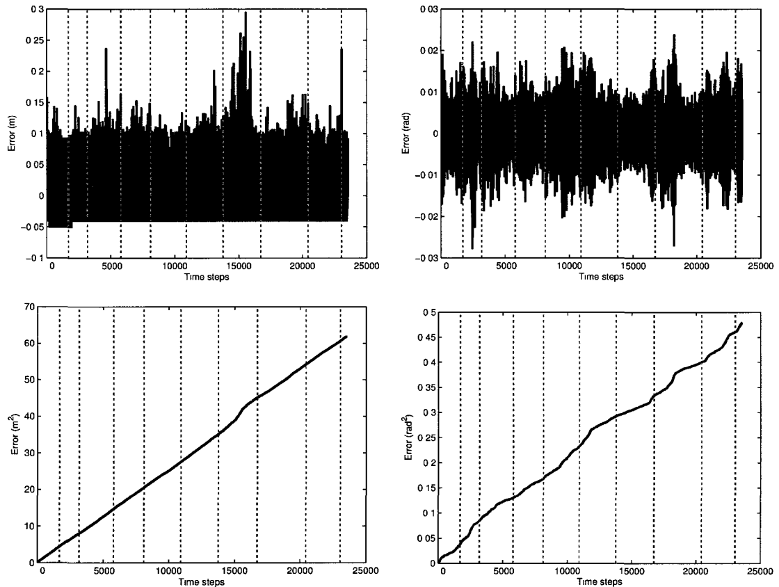
Figure 5.8: MobotSim localization error e_2 and cumulative e_2^2 with \mathbf{Q}_1 noise.
