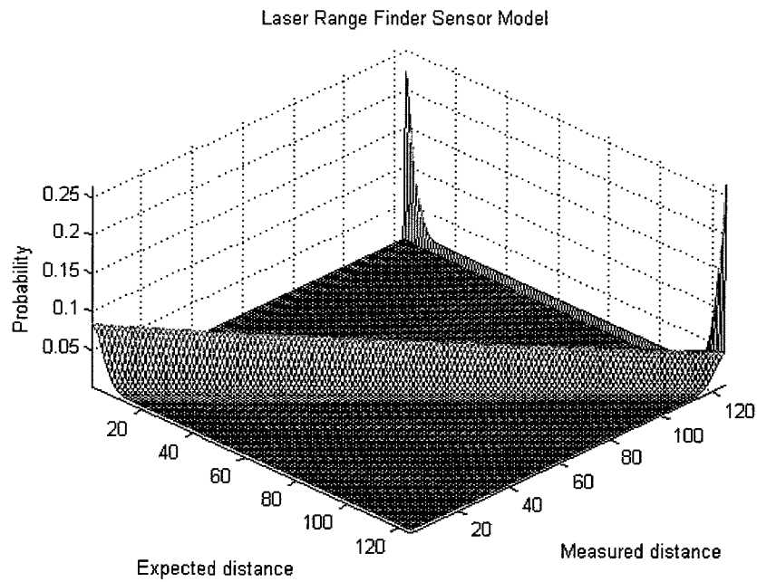
Figure 3.7: Laser Rangefinder Sensor Model.
