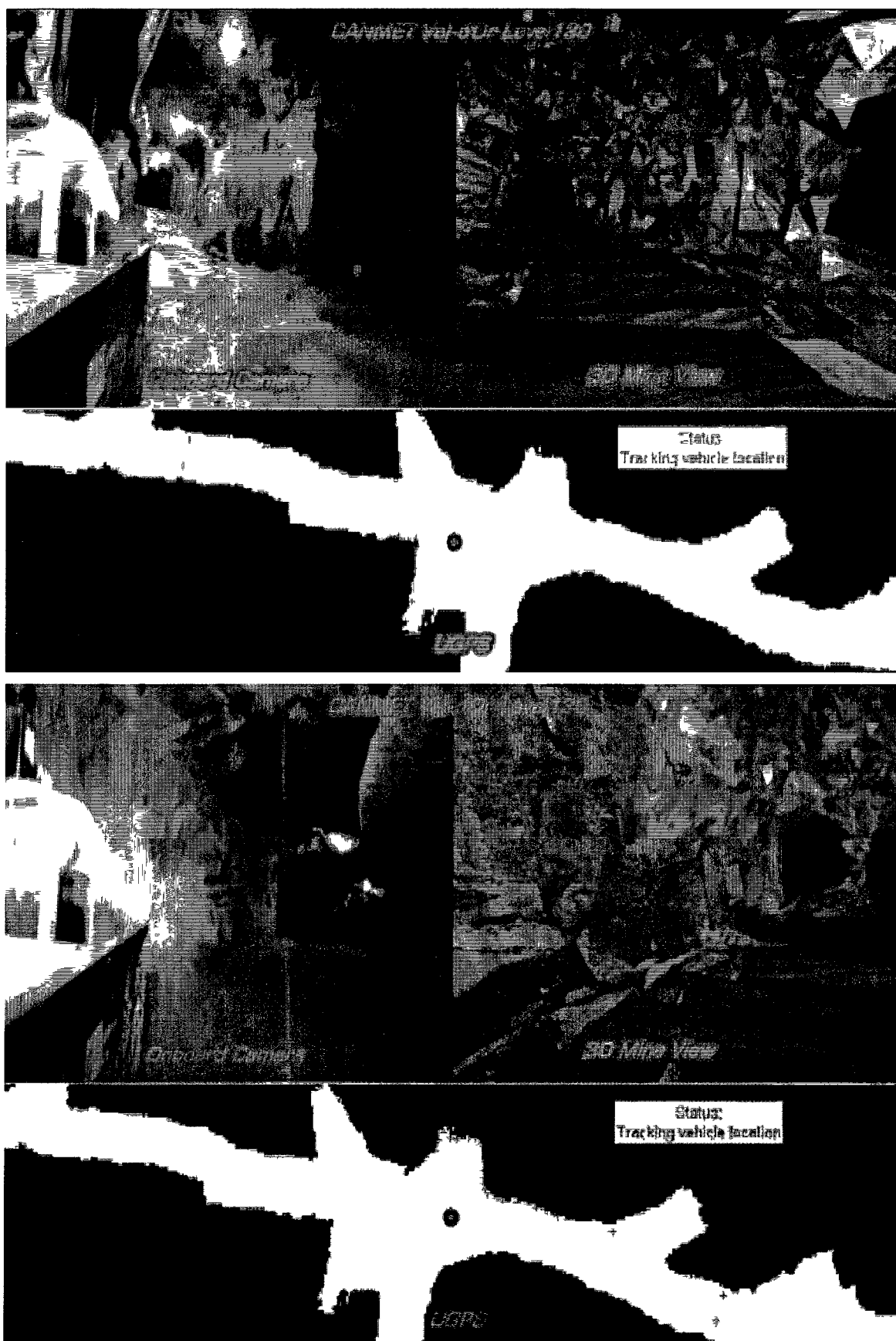
Figure 5.33: CANMET offline localization synchronized with camera and 3D map
