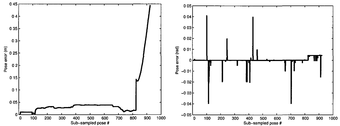
Figure 5.3: MobotSim stitched global map pose errors e_1 .
