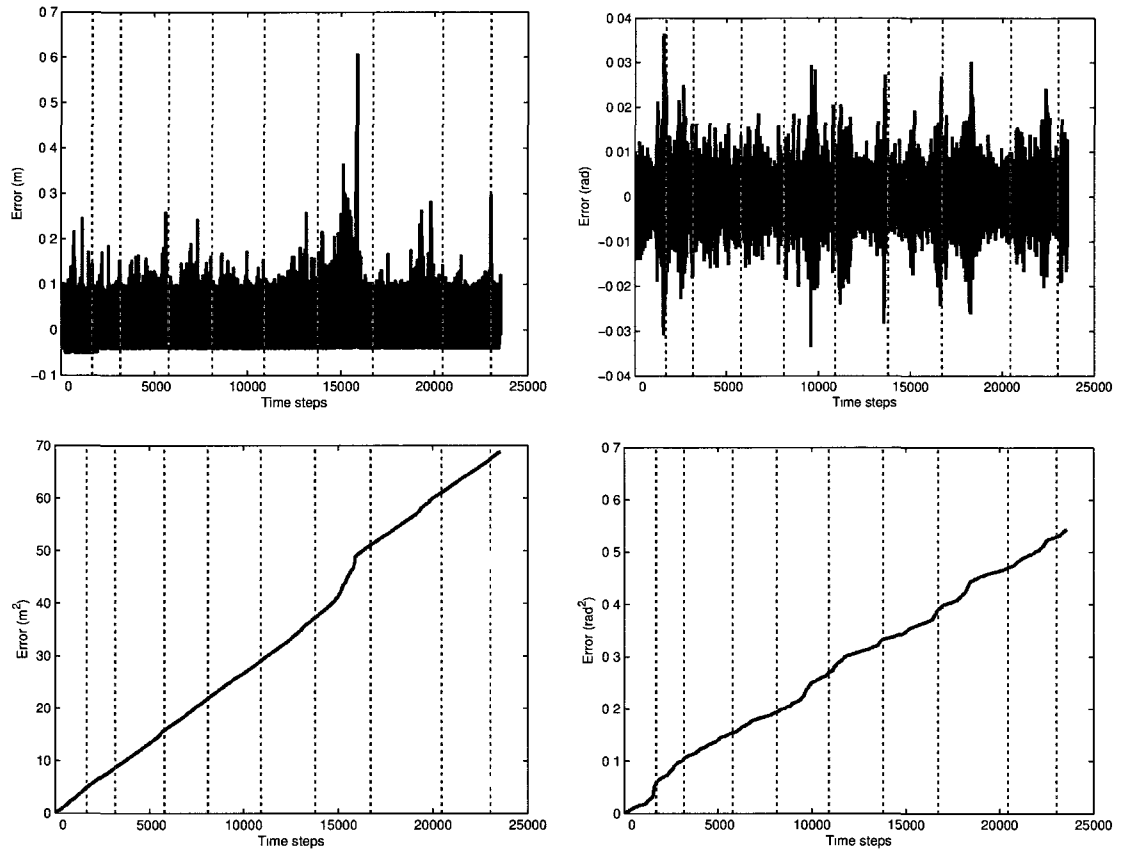
Figure 5.21: MobotSim localization error e_2 and cumulative e_2^2 with Q_1 noise.
