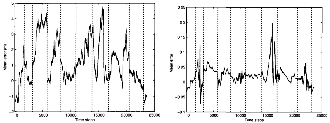
Figure 5.23: MbotSim localization node map reference error e_4 and e_5 with Q_1 noise.
