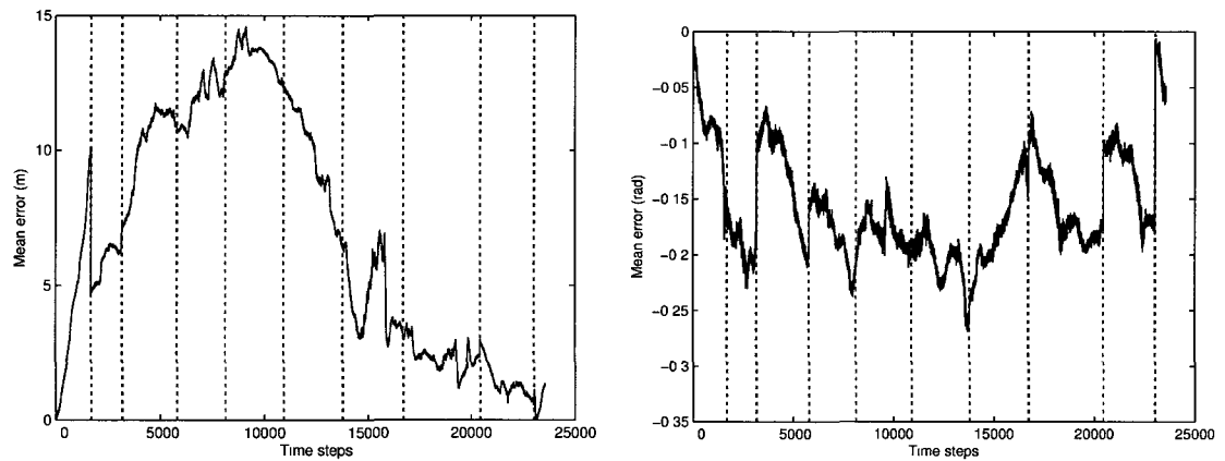
Figure 5.19: MobotSim localization global error e_1 with Q_1 noise.
