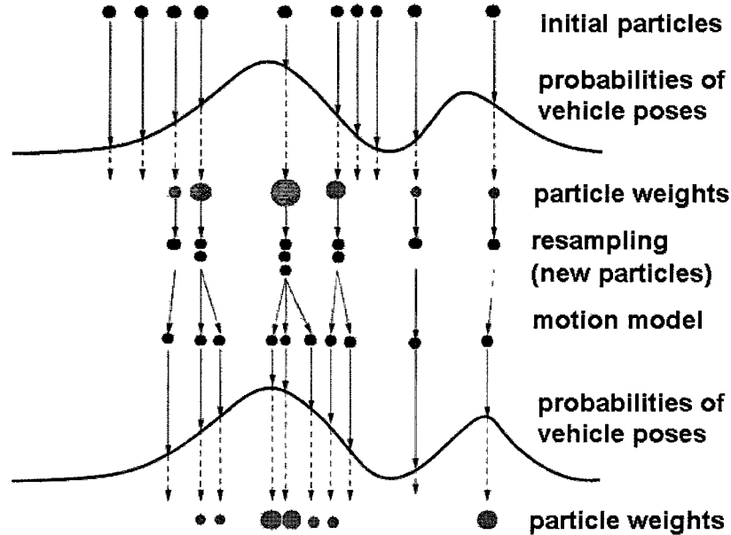
Figure 3.9: Particle filter resampling.
