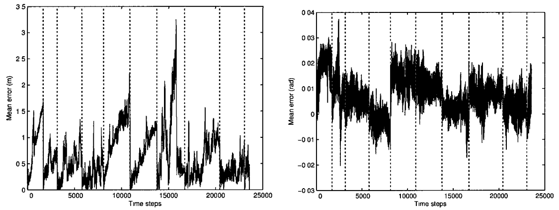
Figure 5.12: MobotSim localization node maps error e_1 with Q_2 noise.
