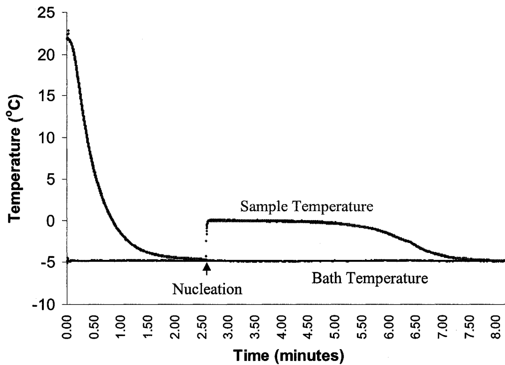
Figure 3. Representative recorded temperature profile with 1.5 mL media in 20 mL scintillation vials placed in a methanol bath at -5 °C.
