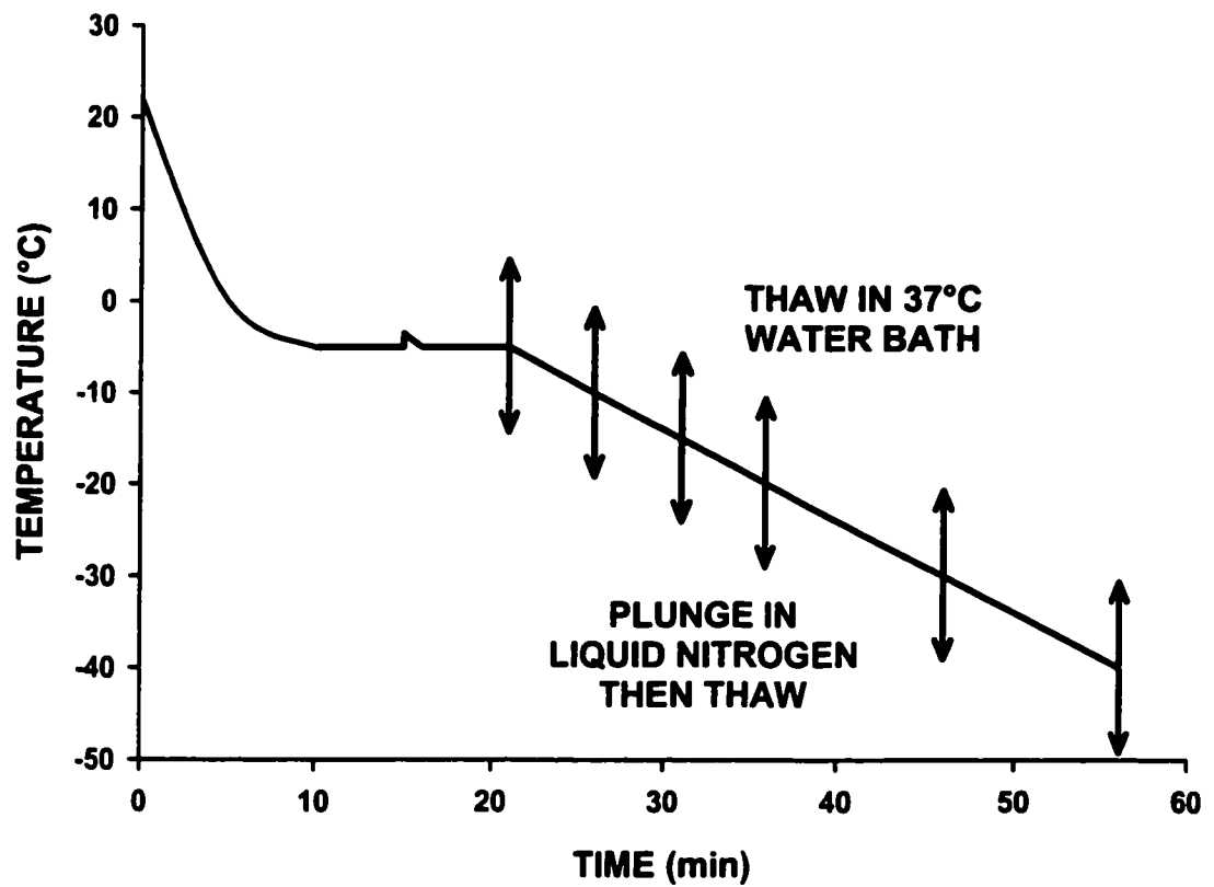
Figure 3.1 – Schematic representation of the graded freezing protocol. This diagram represents samples that would be nucleated at -5°C and then cooled at 1°C/min.
