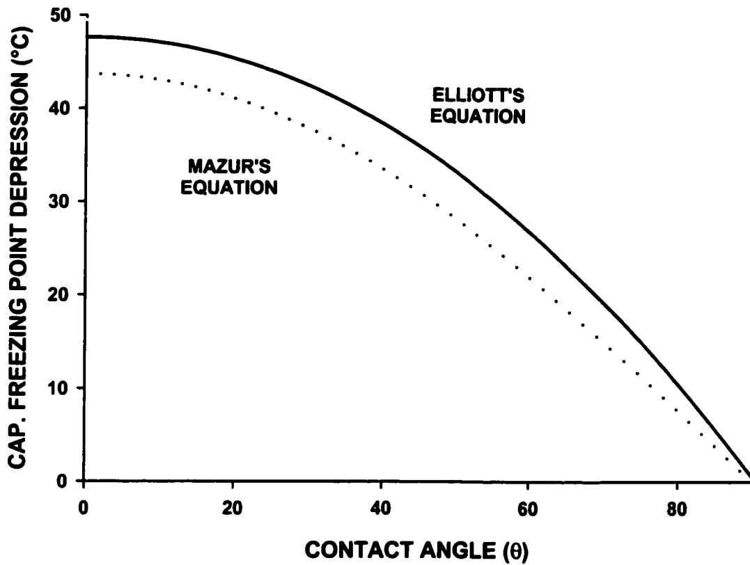
Figure 5.2 – Error associated with the use of Mazur’s approximate equation. Mazur’s equation is compared to the equation derived by Elliott (Equation 5-2). The capillary freezing point depression is calculated as a function of contact angle for a pore radius of 7.5 Å.
