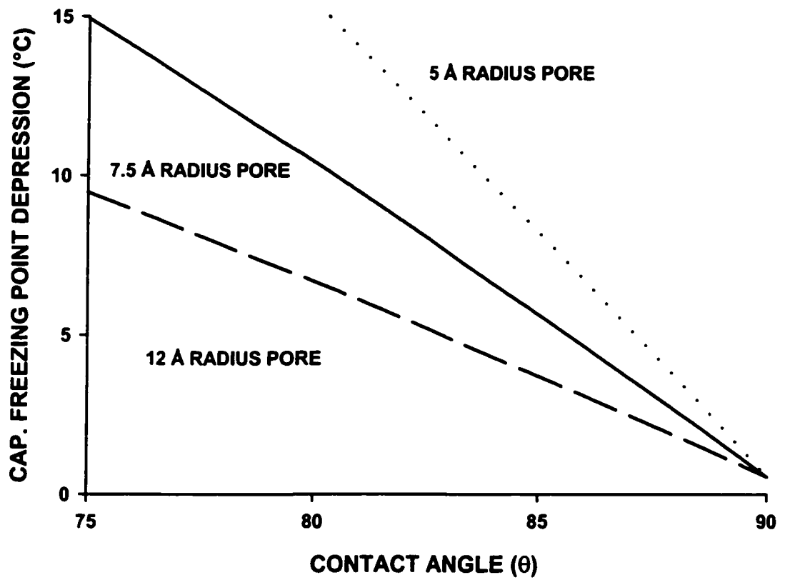
Figure 5.4 – Capillary freezing point depression as a function of contact angle for three pores with defined radii.
