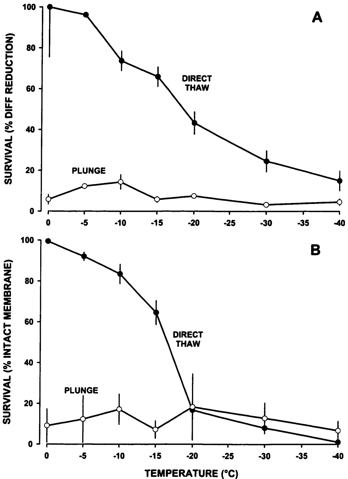
Figure 3.5 – Response of V-79W single attached cells to graded freezing. Samples were nucleated at -5^{\circ}\text{C} , held for 5 min, cooled at 1^{\circ}\text{C}/\text{min} and either thawed directly or plunged into liquid nitrogen. The samples were assessed for metabolic activity (A) and membrane integrity (B). Mean \pm SEM ( n=6 ).
