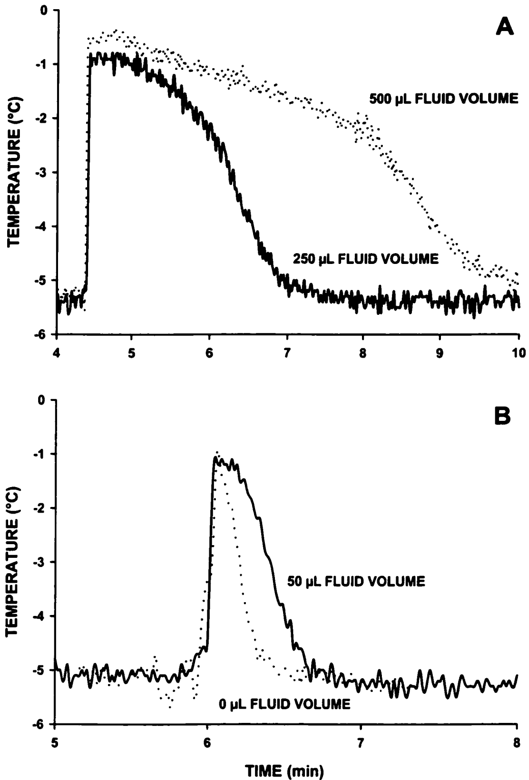
Figure 3.3 – An enlarged view of the nucleation region of the simulated temperature profile for samples in 15 x 45 mm glass vials subjected to a graded freeze. The samples were nucleated at -5°C and held for 5 min before being cooled at 1°C/min. The vials contained either 500 and 250 μL (A) or 50 and 0 μL (B) of tissue culture media.
