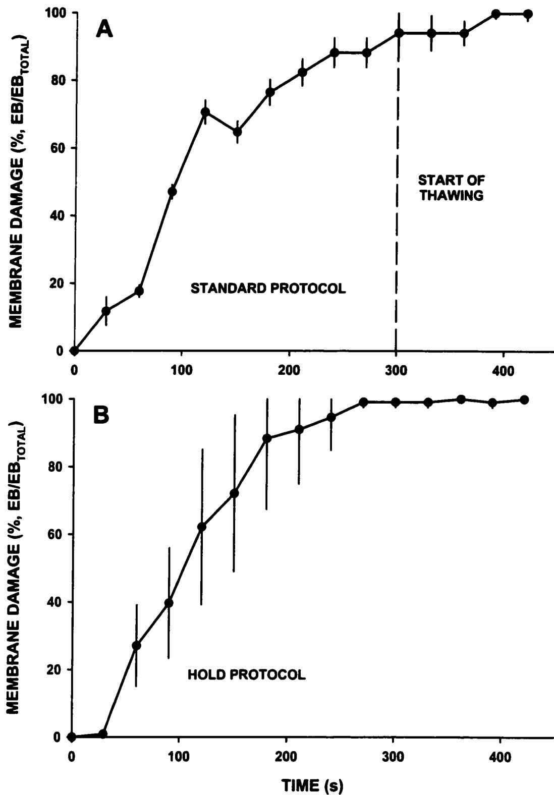
Figure 4.11 – Kinetics of membrane damage detection for MDCK monolayers. Data was collected during a standard cryomicroscopy protocol (A) or a modified protocol where the sample was held at -10^{\circ}\text{C} for 15 min (B). Mean \pm SEM ( n=6 ).
