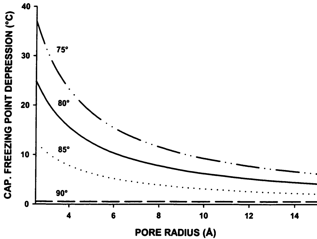
Figure 5.3 – Capillary freezing point depression as a function of pore radius for various contact angles.
